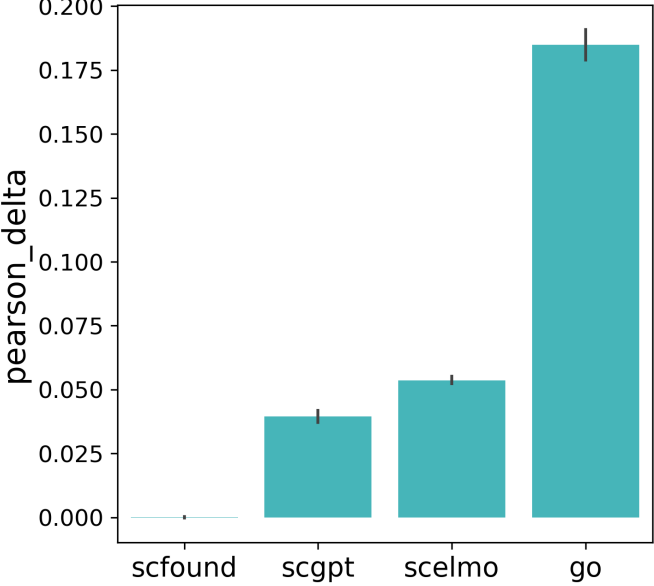
REACTOME
