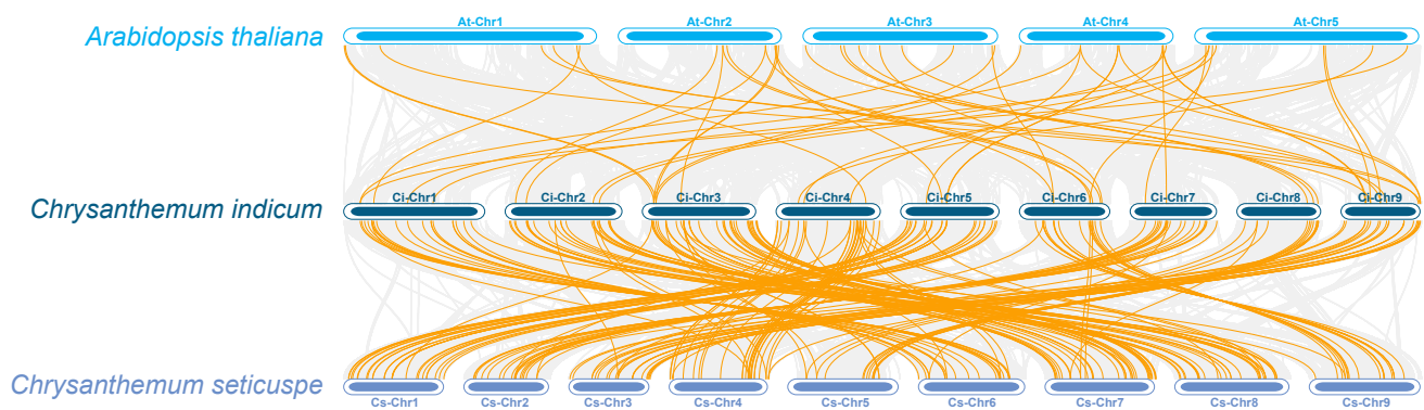
Fig. S3. Collinearity analysis between the CYP450 genes of C. indicum and two representative plant species. The grey lines in the background indicate collinear blocks between C. indicum genome and other plant species genomes, while the orange lines highlight syntenic CYP450 gene pairs.
