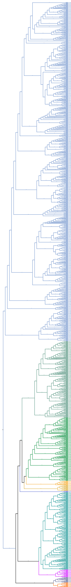
Fig. S1. Phylogenetic analysis of CYP450 genes in Chrysanthemum indicum , Arabidopsis thaliana , Populus trichocarpa , and Oryza sativa .
