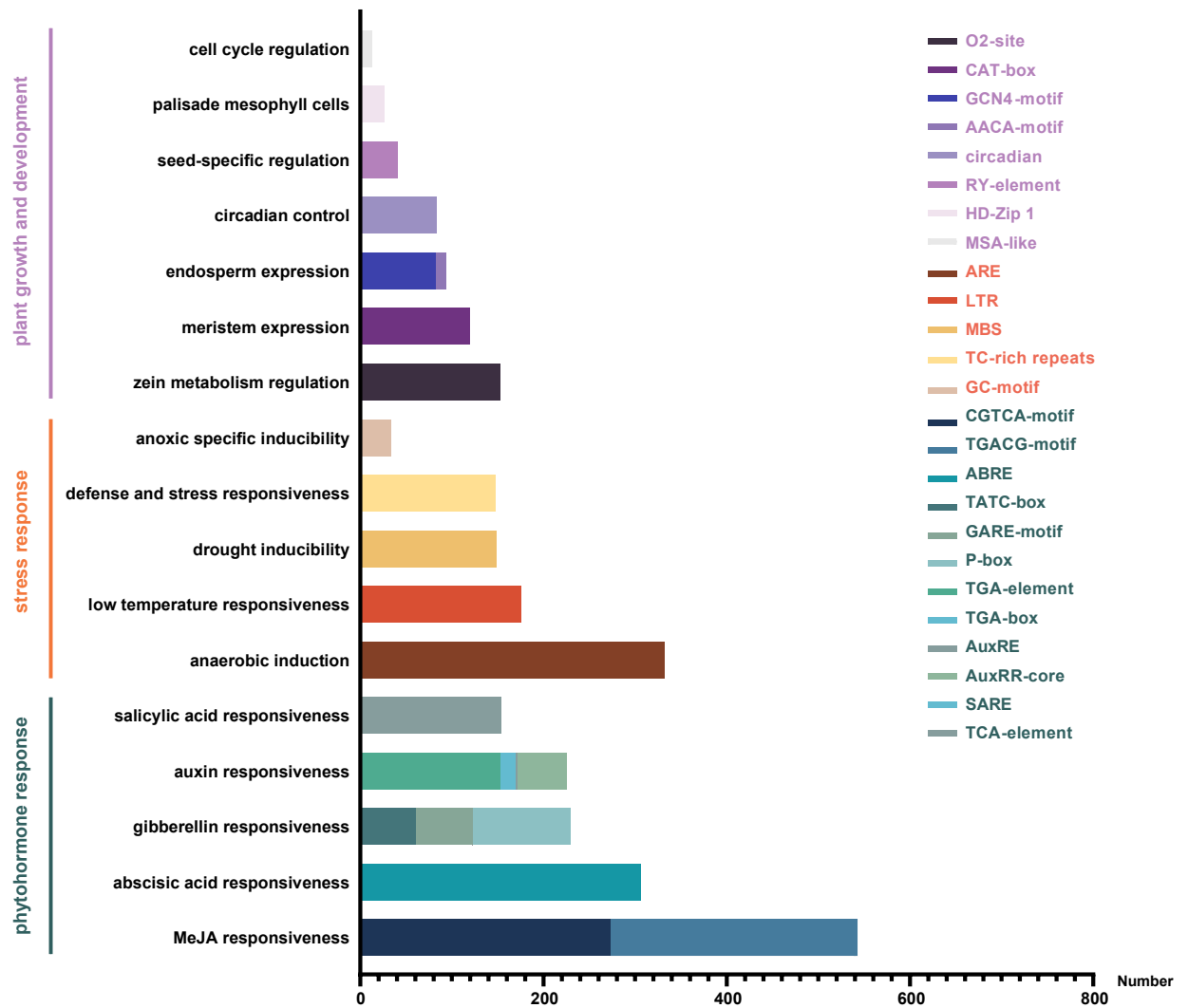
Fig. S4. Different types of cis -elements of CiCYP450 genes.
