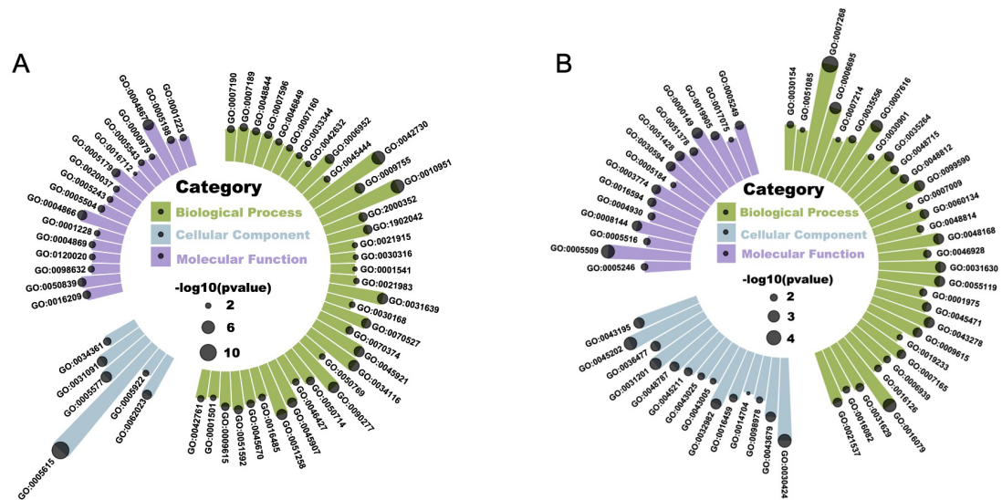
Figure S5. Bar plot of GO terms (Top 60) enriched for hypothalamus (A) and pituitary (B) differentially expressed genes. Different colors represent different categories, and the size of the bubbles at the top of the bars indicates the significance levels.
