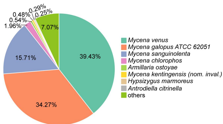
Fig.S4 NR functional annotation of Mycena sp. L02 genome
