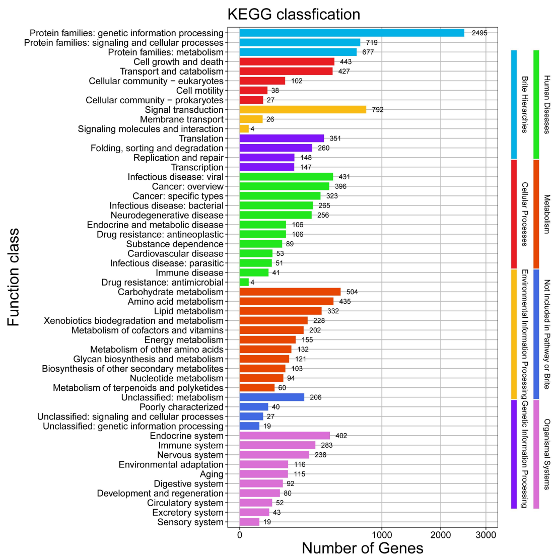
Fig. S2 KEGG pathway annotation of Mycena sp. L02 genome.
