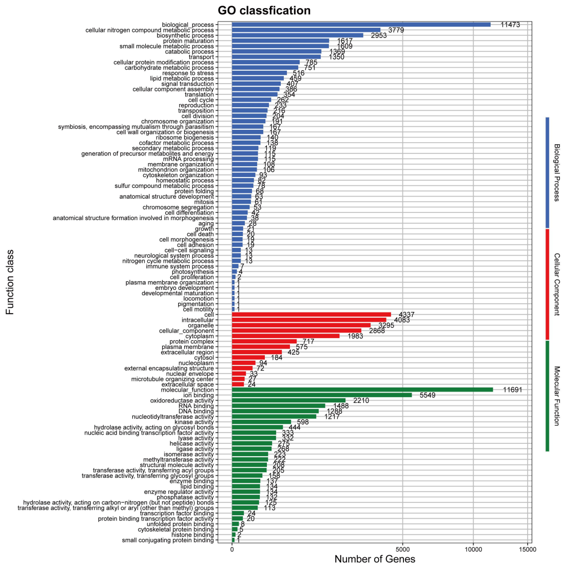
Fig. S1 GO functional annotation of Mycena sp. L02 genome.
