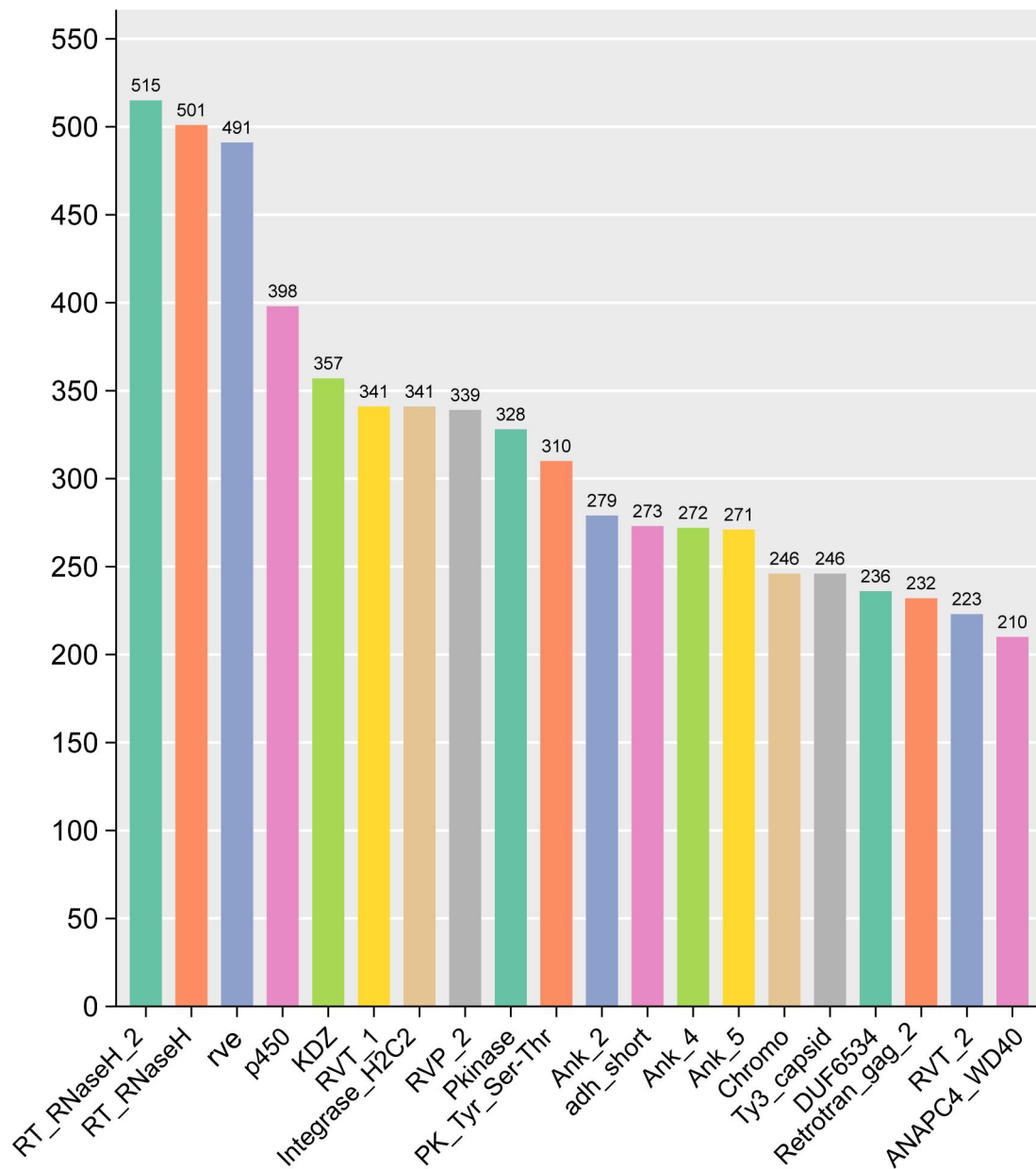
Fig. S3 Pfam functional annotation of Mycena sp. L02 genome
