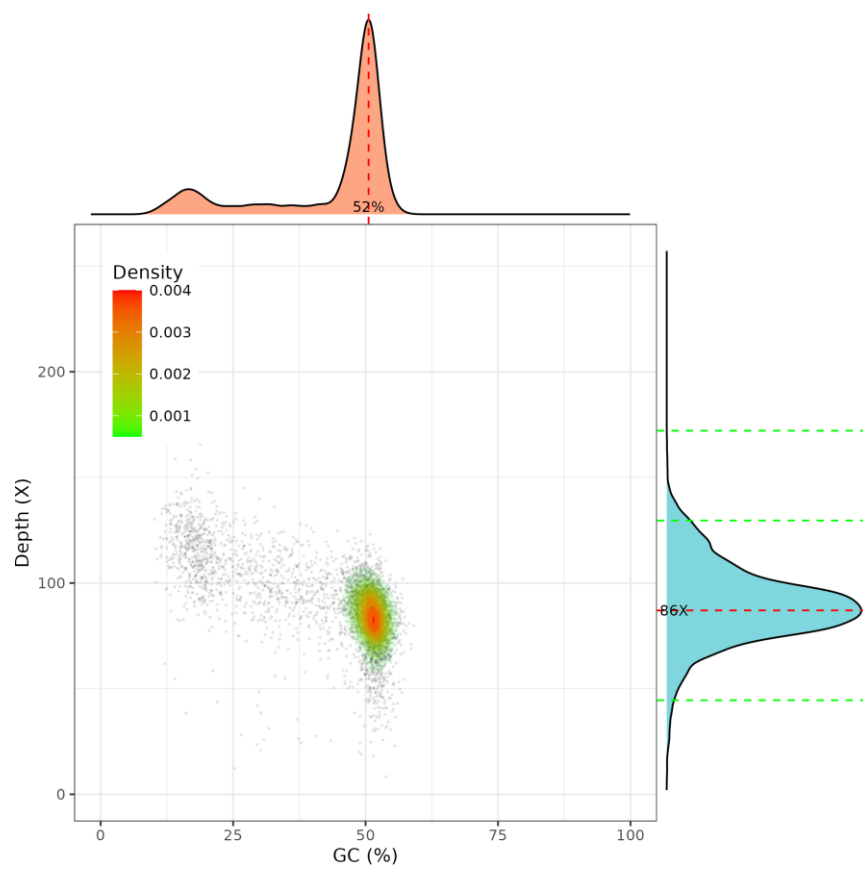
Supplementary Fig. 2 GC content and sequencing depth of the final genome assembly.
