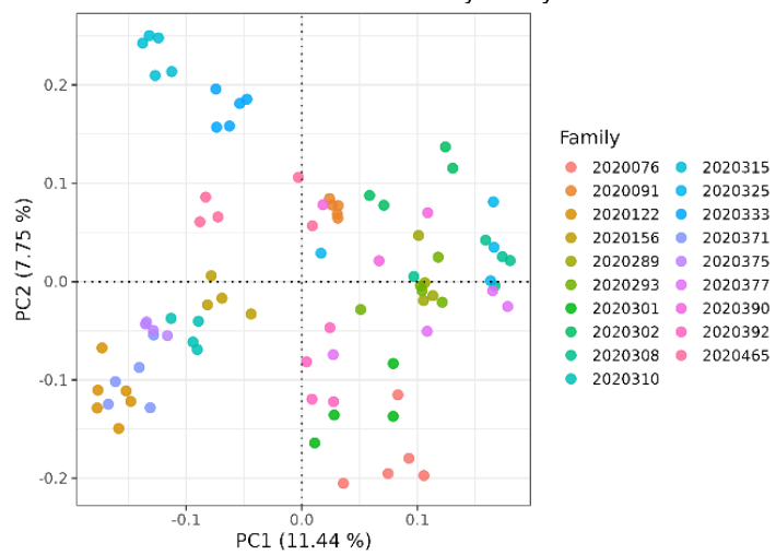
PCA of 85 individuals - coloured by family
