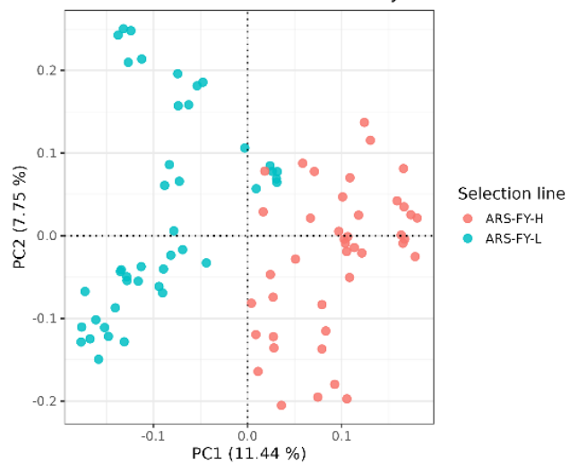
PCA of 85 individuals - coloured by selection line
