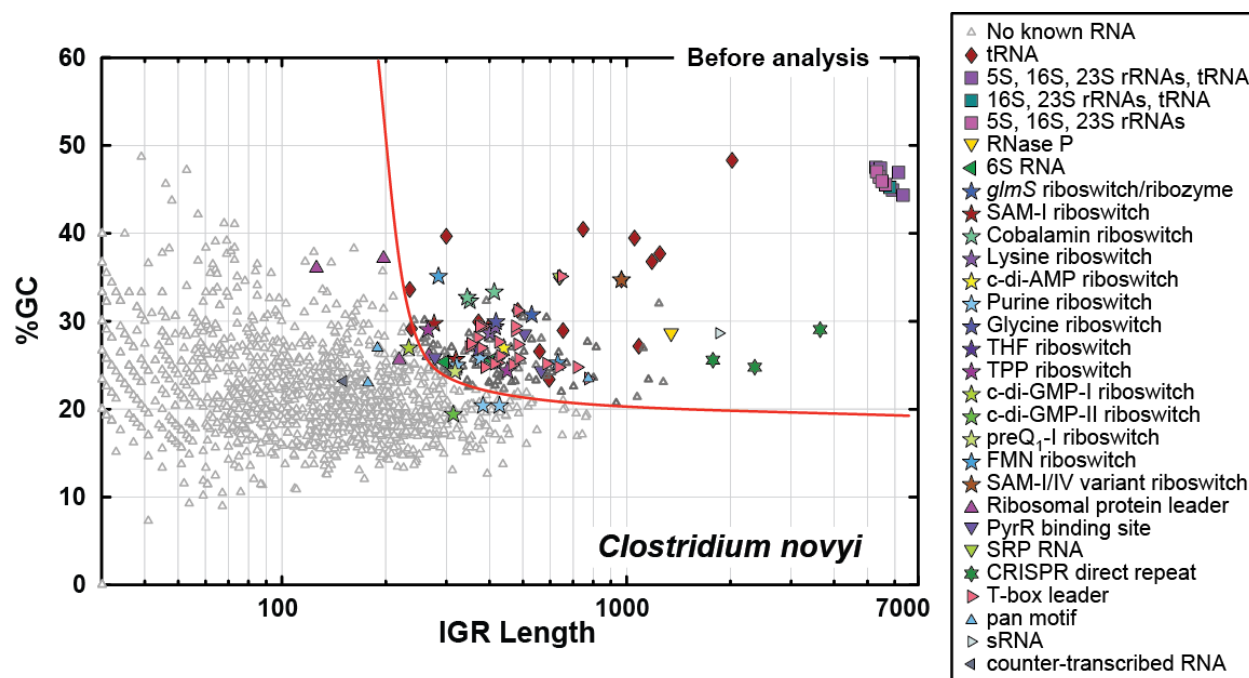
Figure S2 | Plots of the IGRs from the C. novyi genome sorted based on IGR length and GC content. Details are as described in the legend to Fig. 2a.
