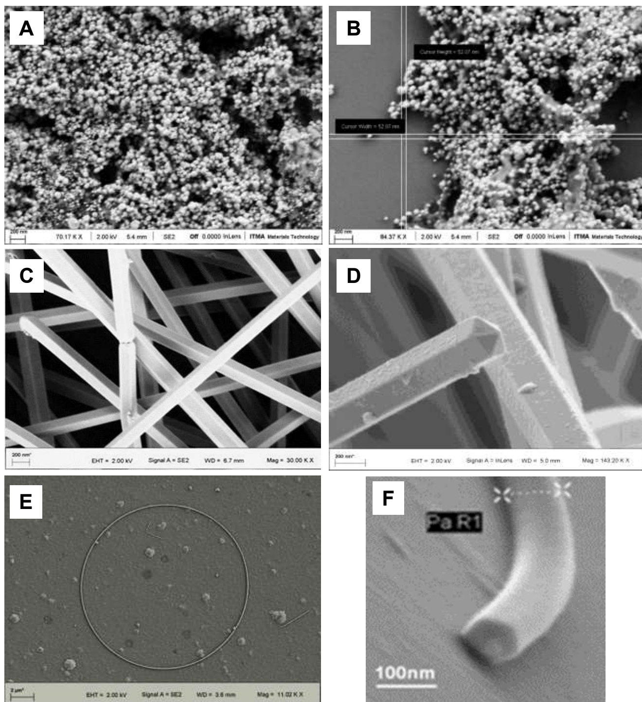
A, B: FEG-SEM Images of silver nanospheres; C,D: FEG-SEM Images of silver nanowires; E,F: FEG-SEM Images of silver nanorings
