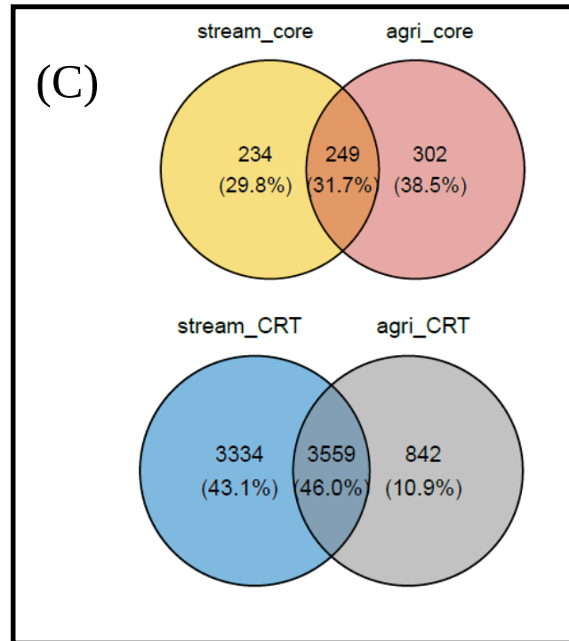
Supplementary Figure S3. Core (agri_core) and CRT (agri_CRT) at agricultural drainage ditch sites. (A) The relative abundances of agri_core and agri_CRT ASVs at the genus level. (B) Area plots represent the fraction of overall community Bray-Curtis dissimilarity (%) attributed to agri_core and agri_CRT over time in 2017 and 2018. The red area represents agri_core's contribution; the green area represents agri_CRT's contribution. (C) Venn diagram plot showing the number of ASVs that are unique or shared by the stream_core and agri_core (top), and the number of ASVs that are unique or shared by the stream_CRT and agri_CRT (bottom). (D) The relative abundance of ASVs in agri_core that were not identified as stream_core under the four land use classes.
