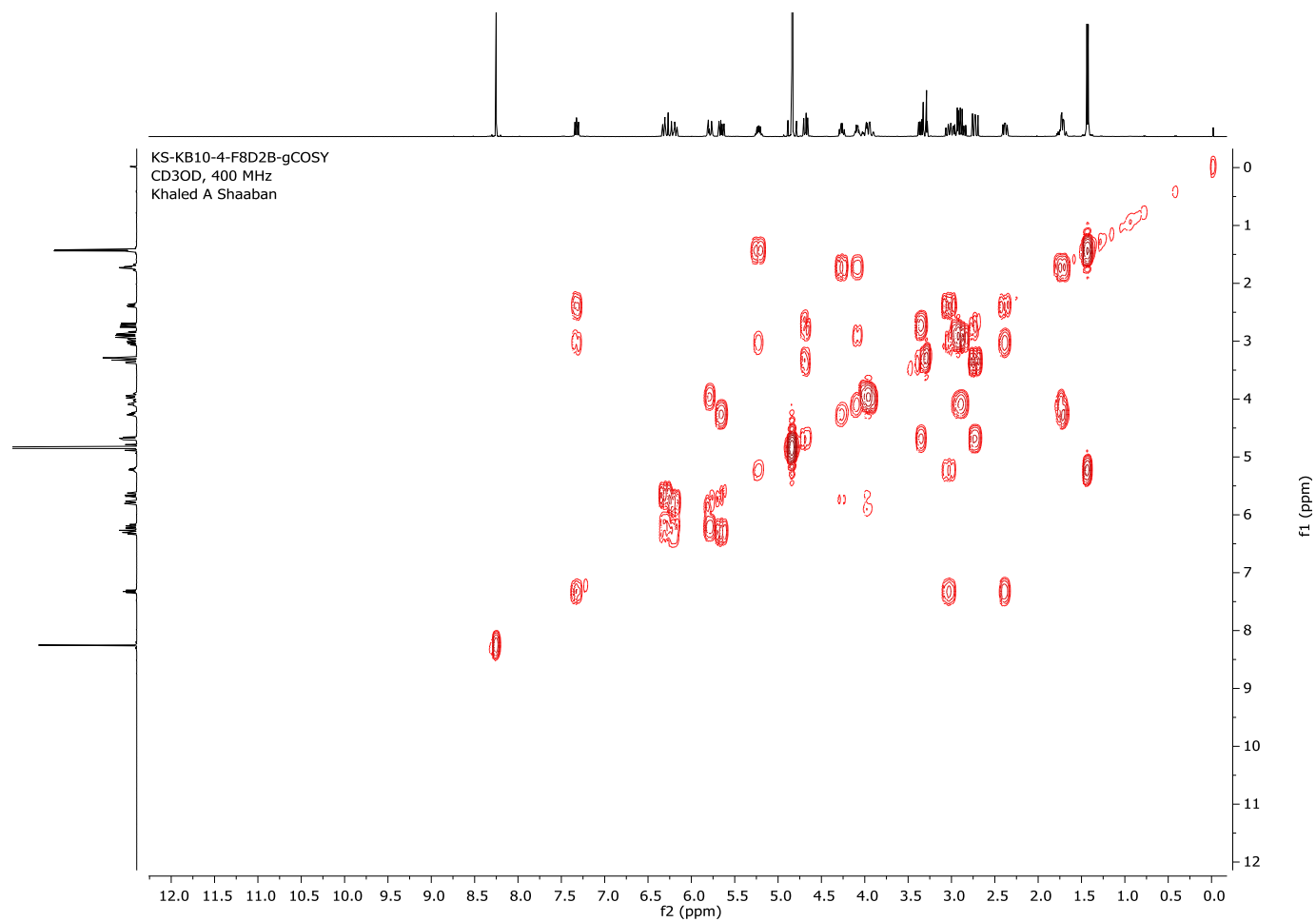
Figure S19: ^1\text{H} , ^1\text{H} -COSY spectrum ( \text{CD}_3\text{OD} , 400 MHz) of griseoviridin (1).
