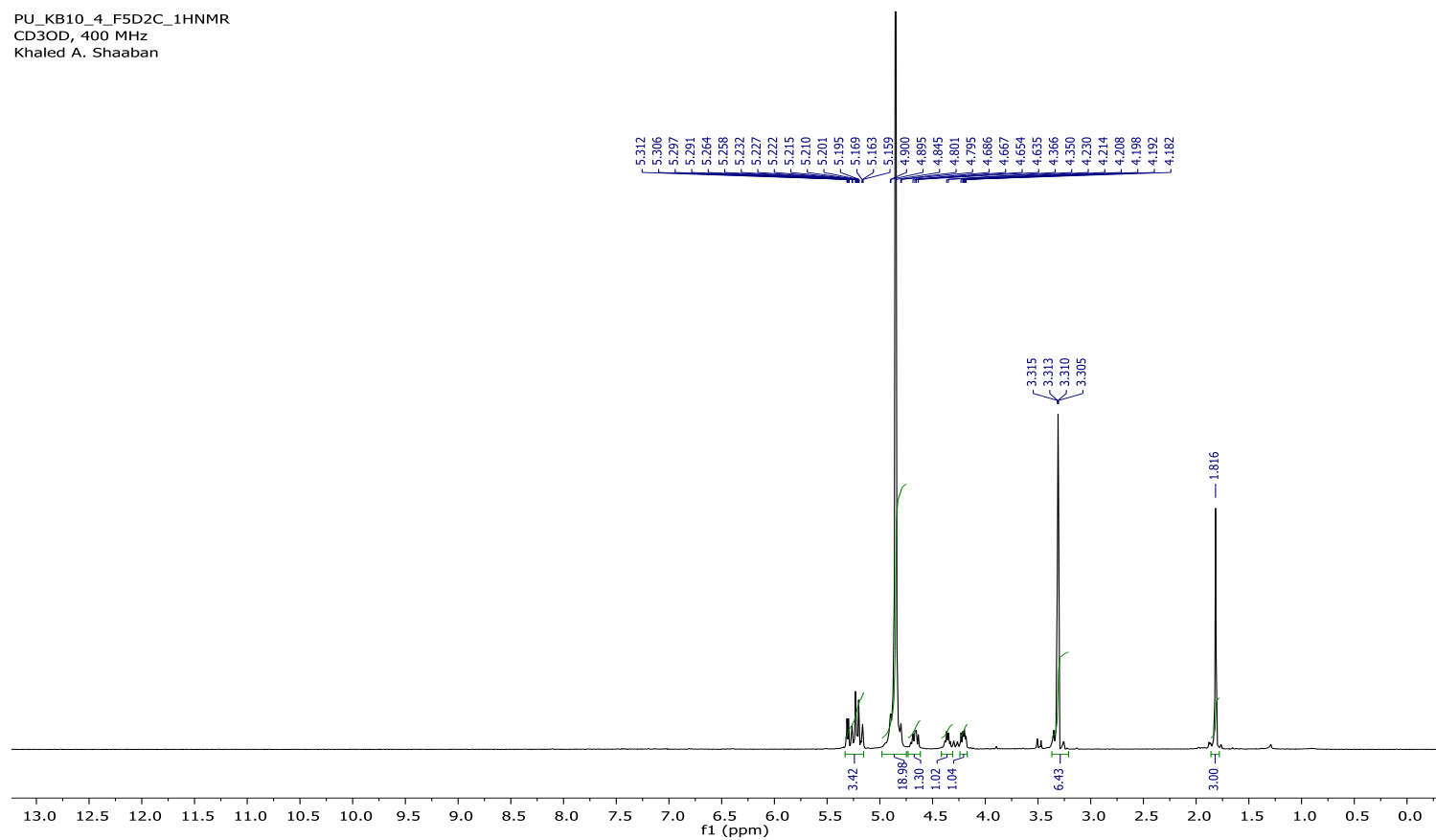
Figure S24: ^1\text{H} NMR spectrum ( \text{CD}_3\text{OD} , 400 MHz) of mitomycin C (2).
