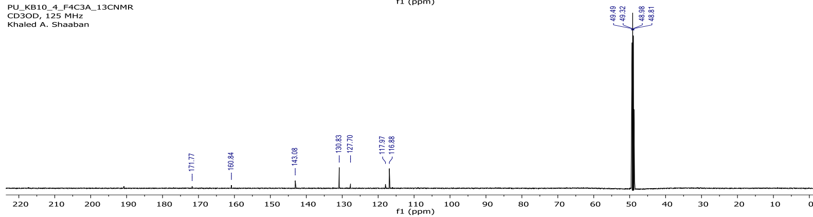
Figure S31: ^1\text{H} (500 MHz) and ^{13}\text{C} (125 MHz) NMR spectra of 4-hydroxycinnamide (3) in \text{CD}_3\text{OD} .
