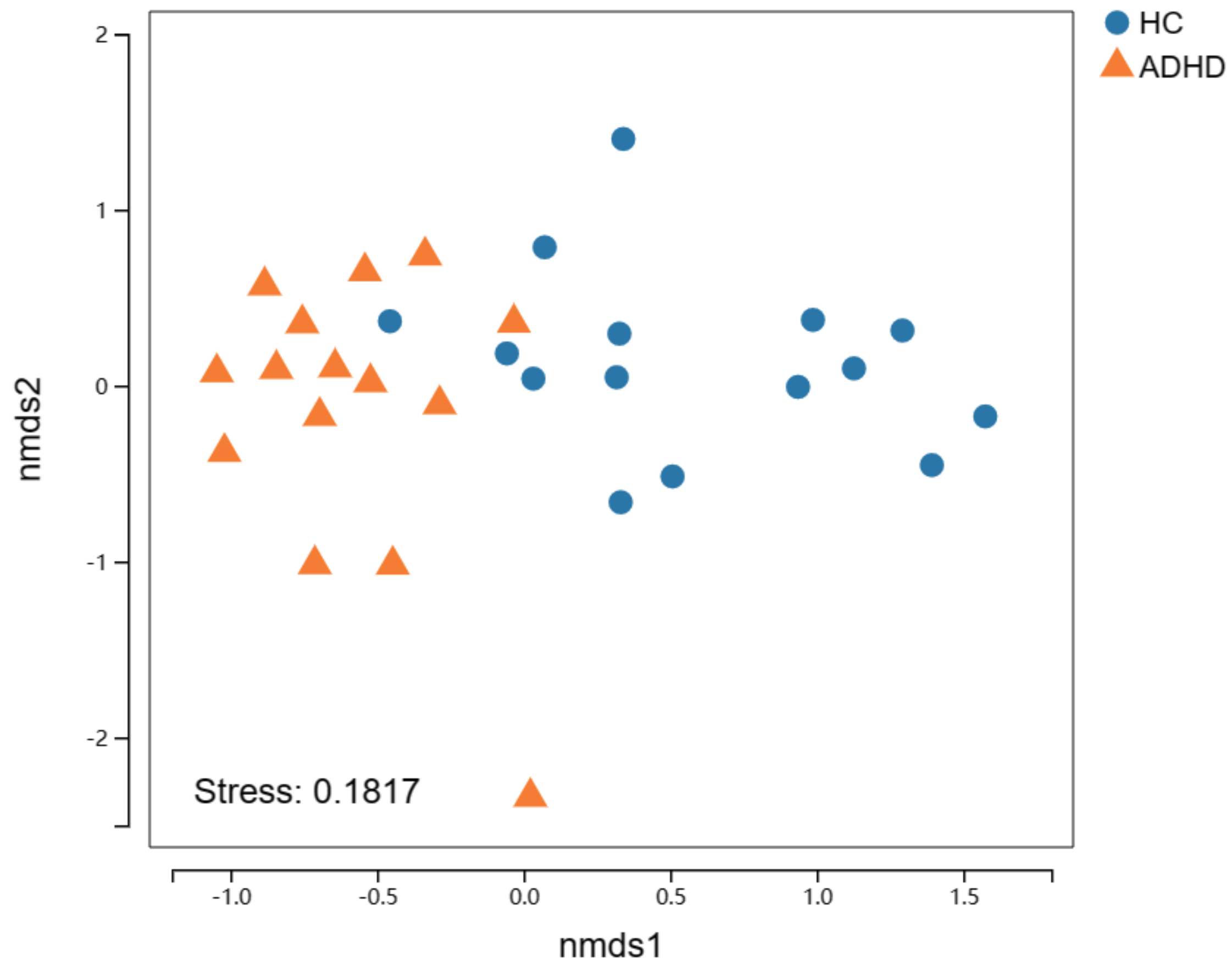
NMDS
