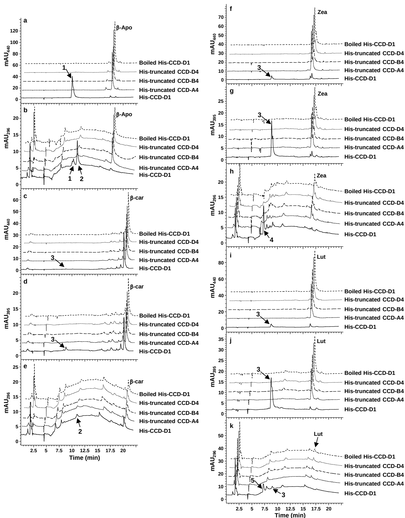
Figure S6. In vitro activities of truncated wheat CCD4 homeologs. \beta -apo-8'-carotenal ( \beta -apo; a,b), \beta -carotene ( \beta -car; c-e), zeaxanthin (Zea; f-h), and lutein (Lut; i-k) were used as substrates in the enzyme assays. Product peaks are indicated by arrows. Absorption and MS spectra of the product peaks are shown in Fig. 3.
