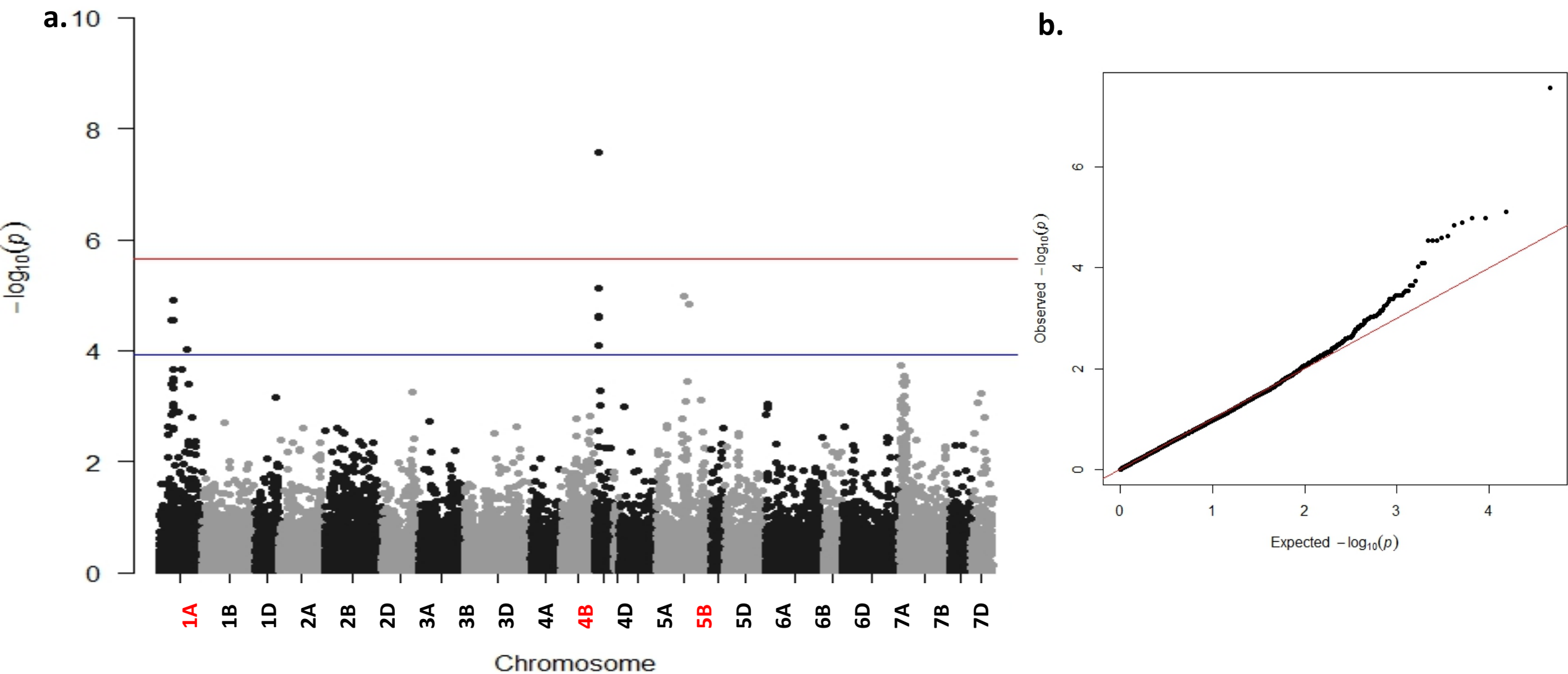
Supplementary Figure 4. a) Manhattan plot displaying SNP marker-trait association identified for plant height in GWAS using winter wheat lines. Redline is significance threshold of 5% Bonferroni correction and blue line is significance threshold of FDR. Chromosomes with names written in red are carrying SNPs significantly associated with plant height. b) Quantile-Quantile (QQ) plot used to evaluate the performance of the mixed linear model used for GWAS for plant height using mixed linear model (MLM+Q-matrix).
