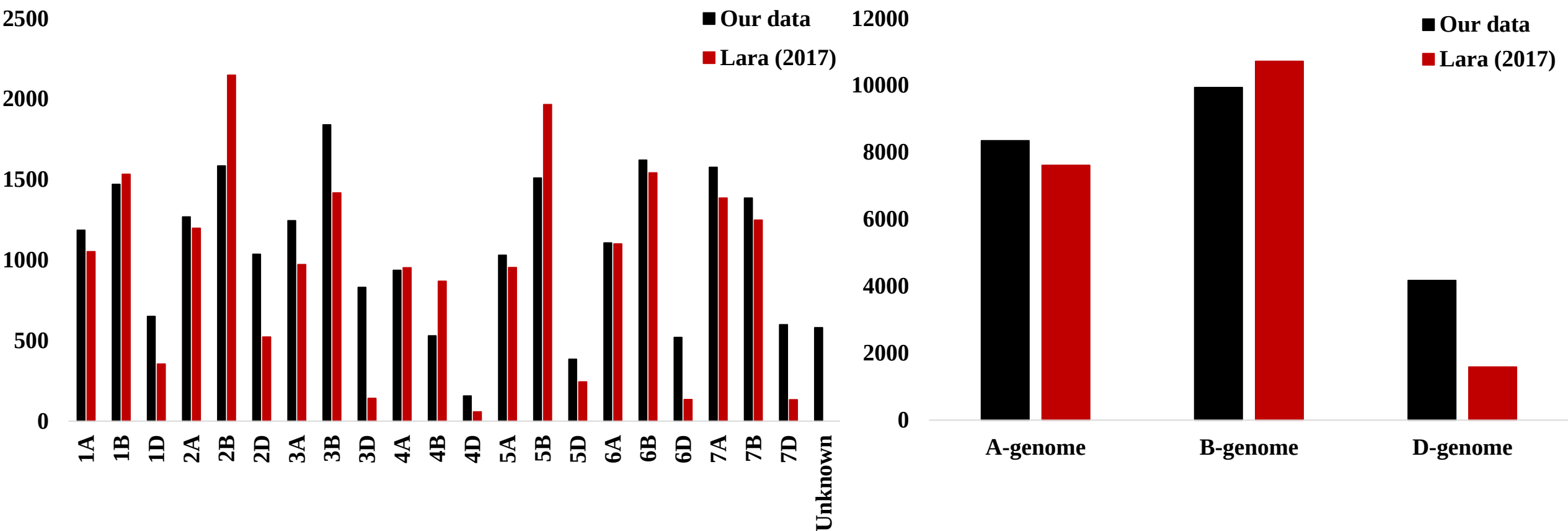
Supplementary Figure 5. The distribution of the SNPs across a) the different wheat chromosomes and b) the different wheat genomes. Black charts representing the number of SNPs used in the present study while red charts represent the number of SNPs used in previous studies (Lara 2017).
