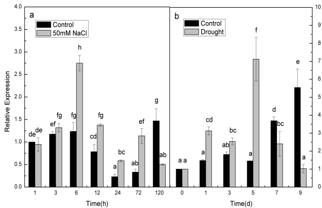
Additional file 3: Expressions of CmLOX08 at various time points under drought (a) and 50 mM NaCl (b) treatments.
