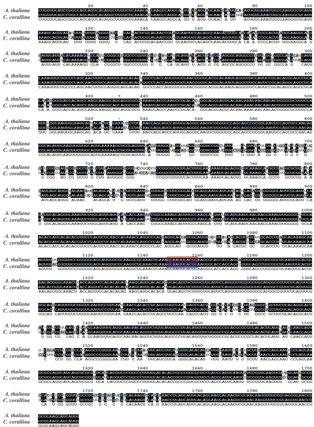
Figure S6. Alignment of 18S rRNA sequences of A. thaliana and C. corallina . The red box indicates the Arabidopsis rRNA sequence at nt positions 1141-1151 to which APUM23 binds, and the blue box shows the identical sequence at nt positions 1148-1158 of 18S rRNA in C. corallina .
