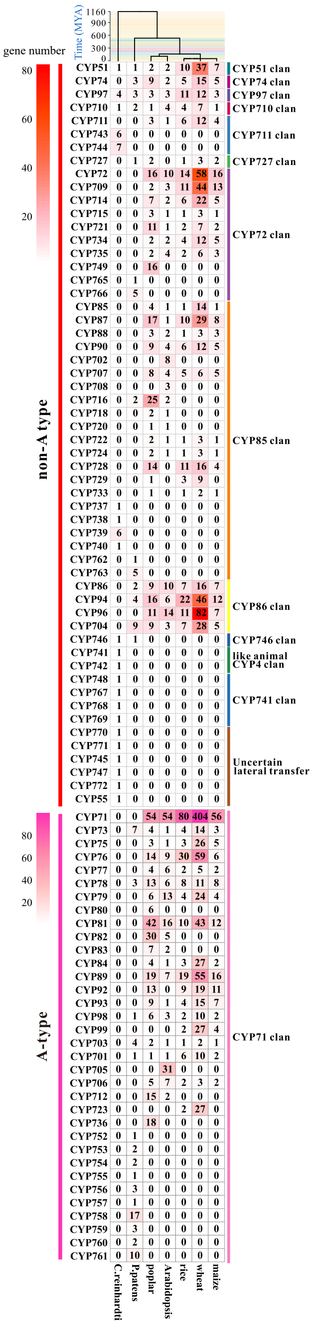
Figure S1. Comparison of CYP450 families among green alga, moss, poplar, Arabidopsis, rice, wheat and maize.
