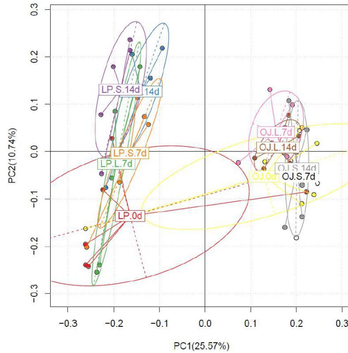
Figure S2. Principal Component Analysis (PCA) in rhizosphere soil microbial communities of shade-tolerant OJ ( Ophiopogon japonicus ) and shade-intolerant LP ( Lolium perenne ) under shade stress. OTUs delimited at 97% similarity.
