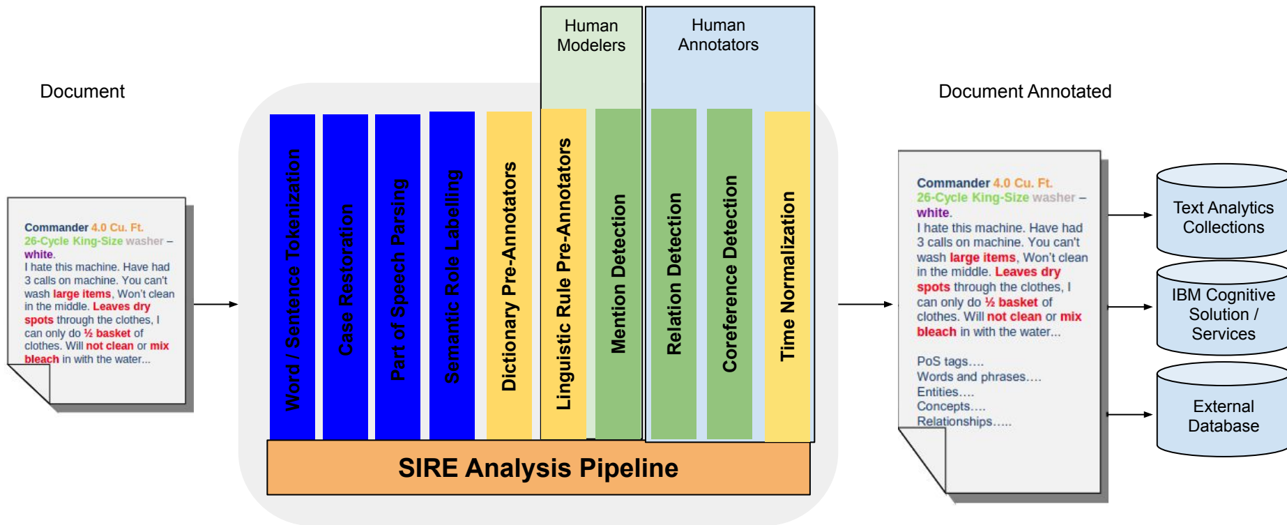
Additional File 5: A schematic representation of the Statistical Information and Relation Extraction (SIRE) pipeline used by Watson.
