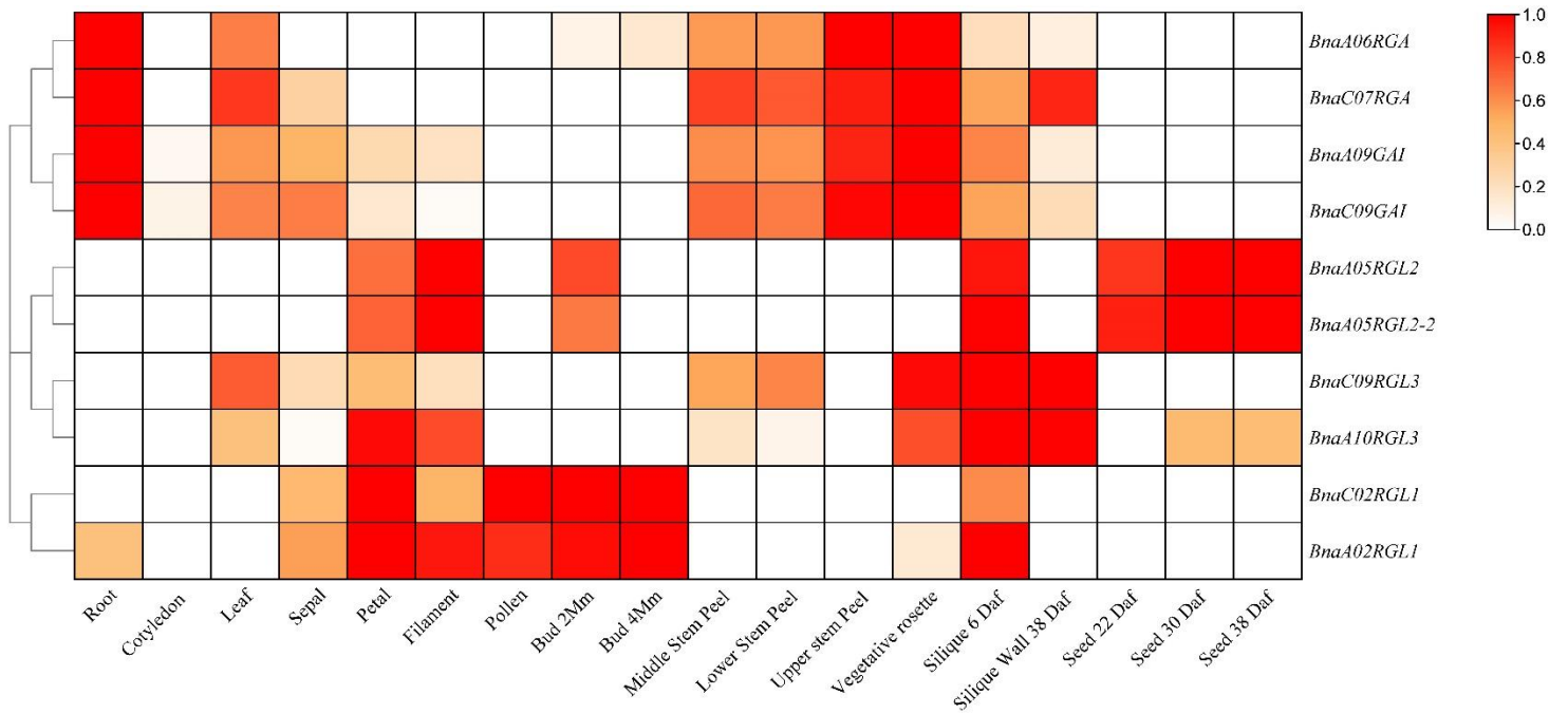
Figure. S4 BnaDELLA s expression at different development stages in different organs by transcriptomic analysis. Expression data were analyzed with log2 normalization. Relative expression levels from high (dark-colored) to low (light color) are represented by the color scale bar (listed in Table S5.1).
