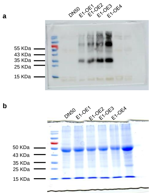
Figure S4. Source data of full gel blot images for figure 1a. a, original gel blot image of figure 1a, upper panel. b, original image of figure 1a, lower panel.
