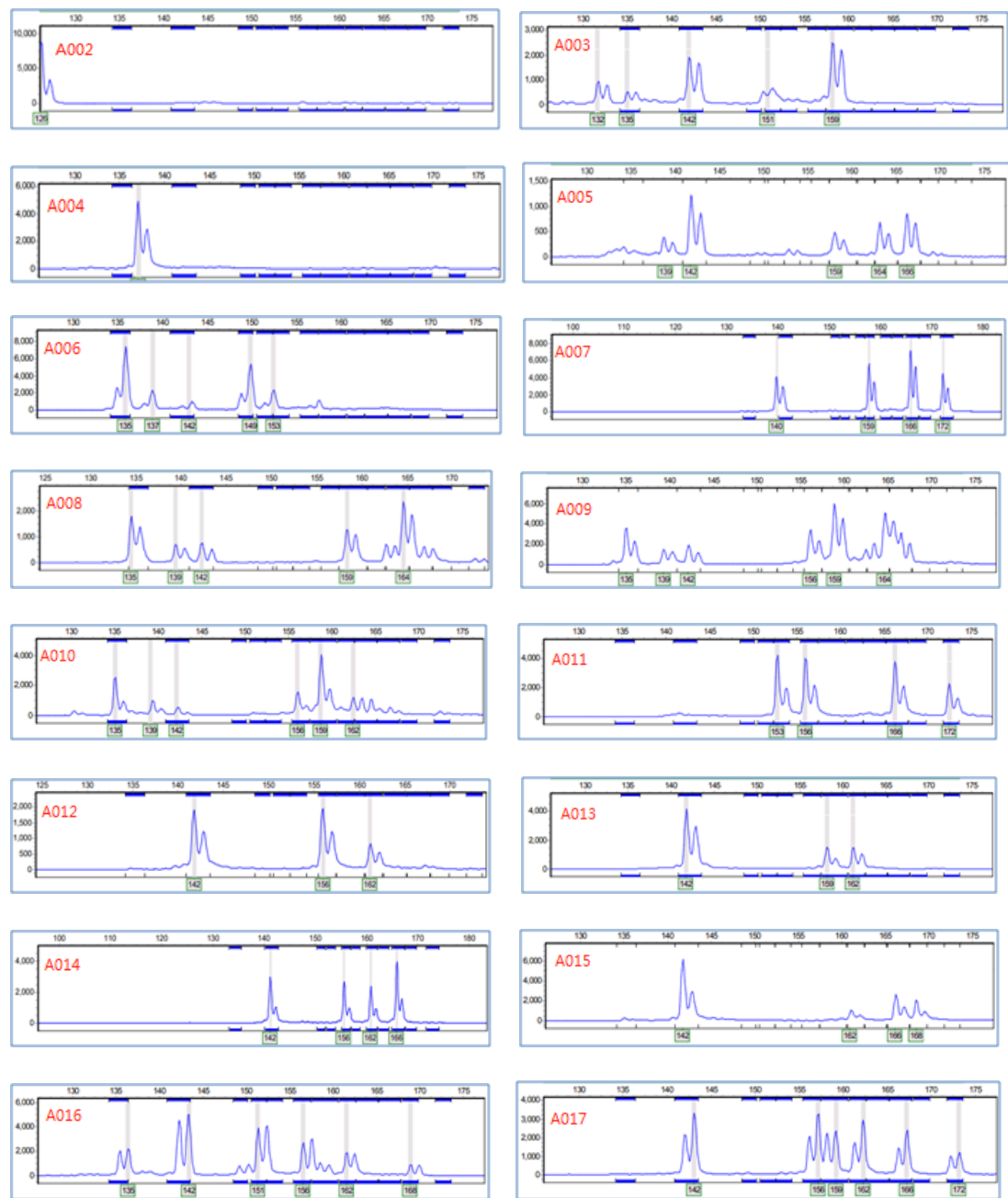
Figure S2. Scanning peak graphs of all 943 genotypes.
