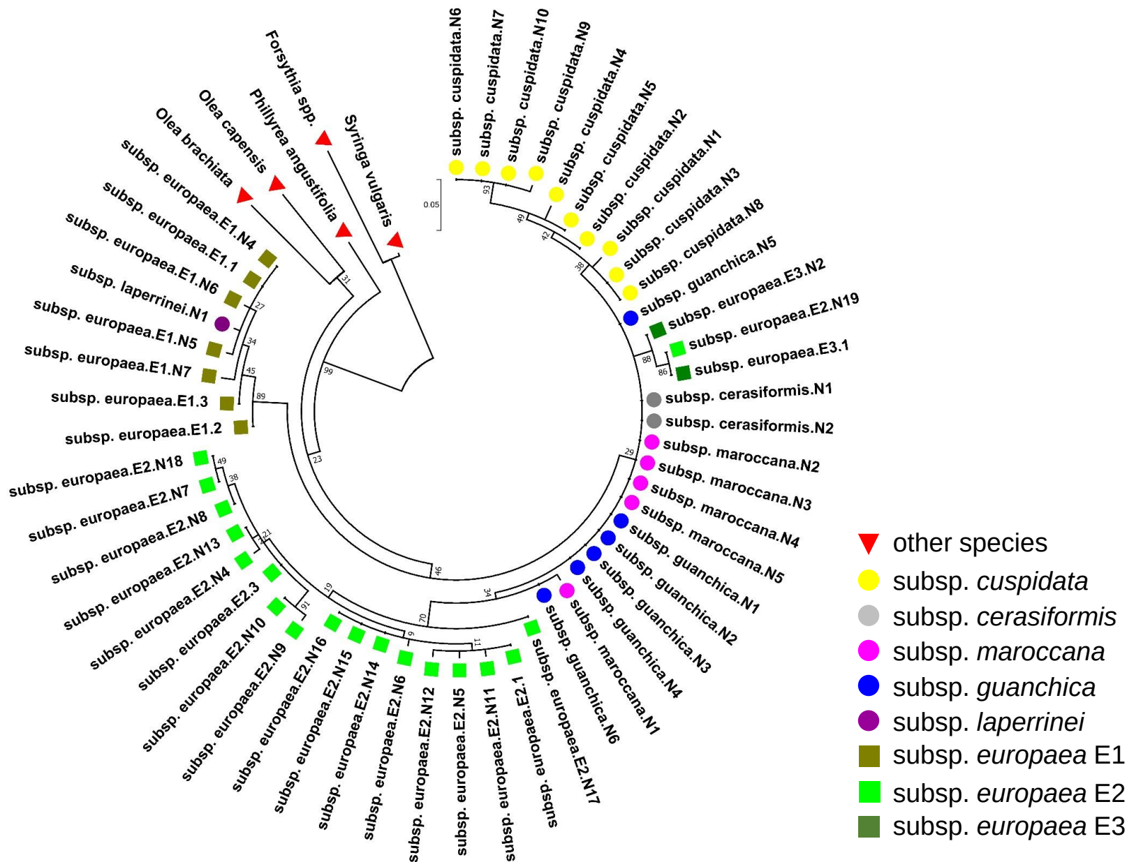
Supplementary Figure S1. Rounded dendrogram derived from the MEGA7 analysis by applying Maximum Likelihood method on the sequences of the 56 different chlorotypes identified.
