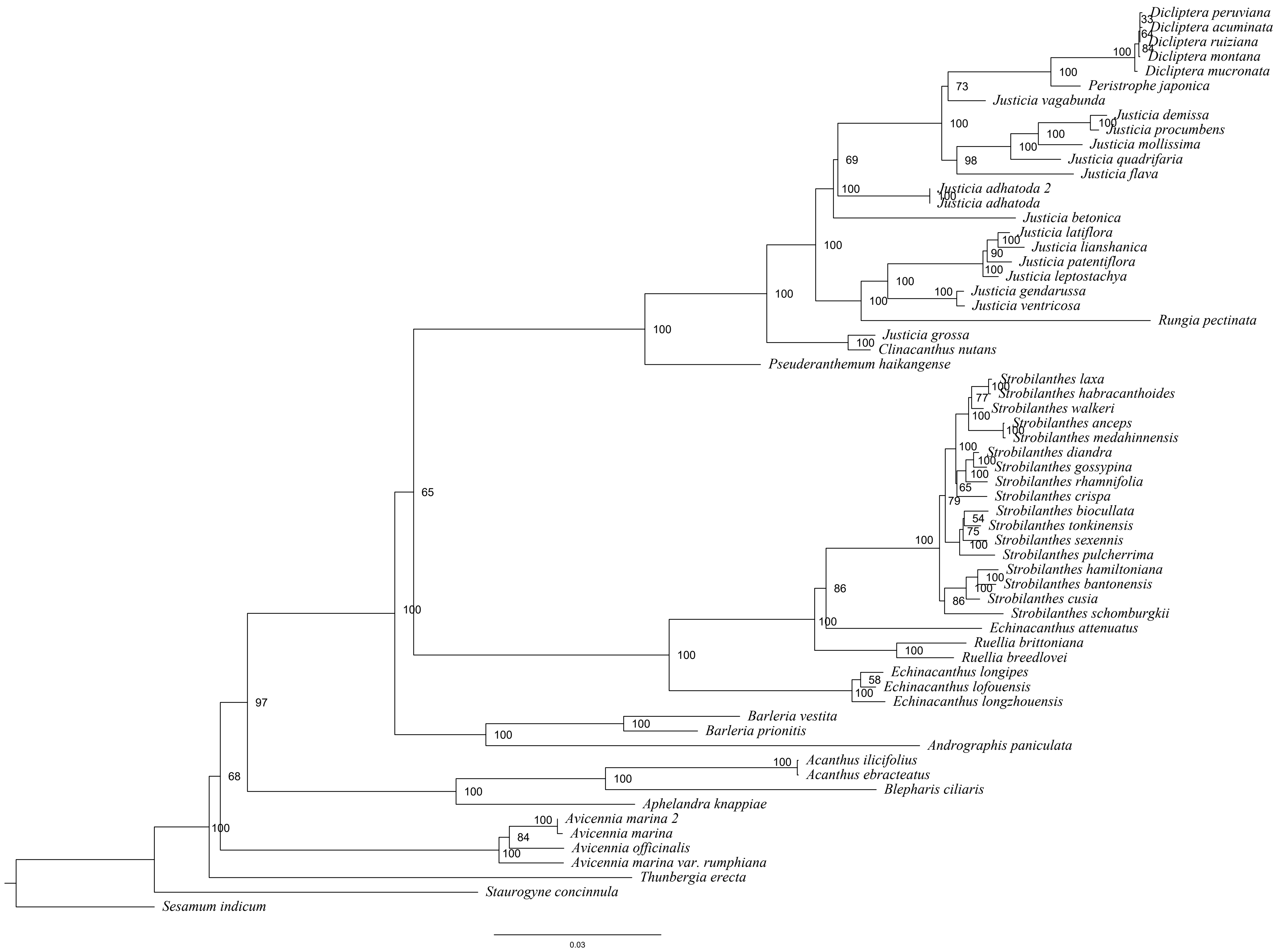
Fig. S5 Phylogenetic reconstruction for Justicia species and other genera of Acanthaceae based on ycf1 gene.
