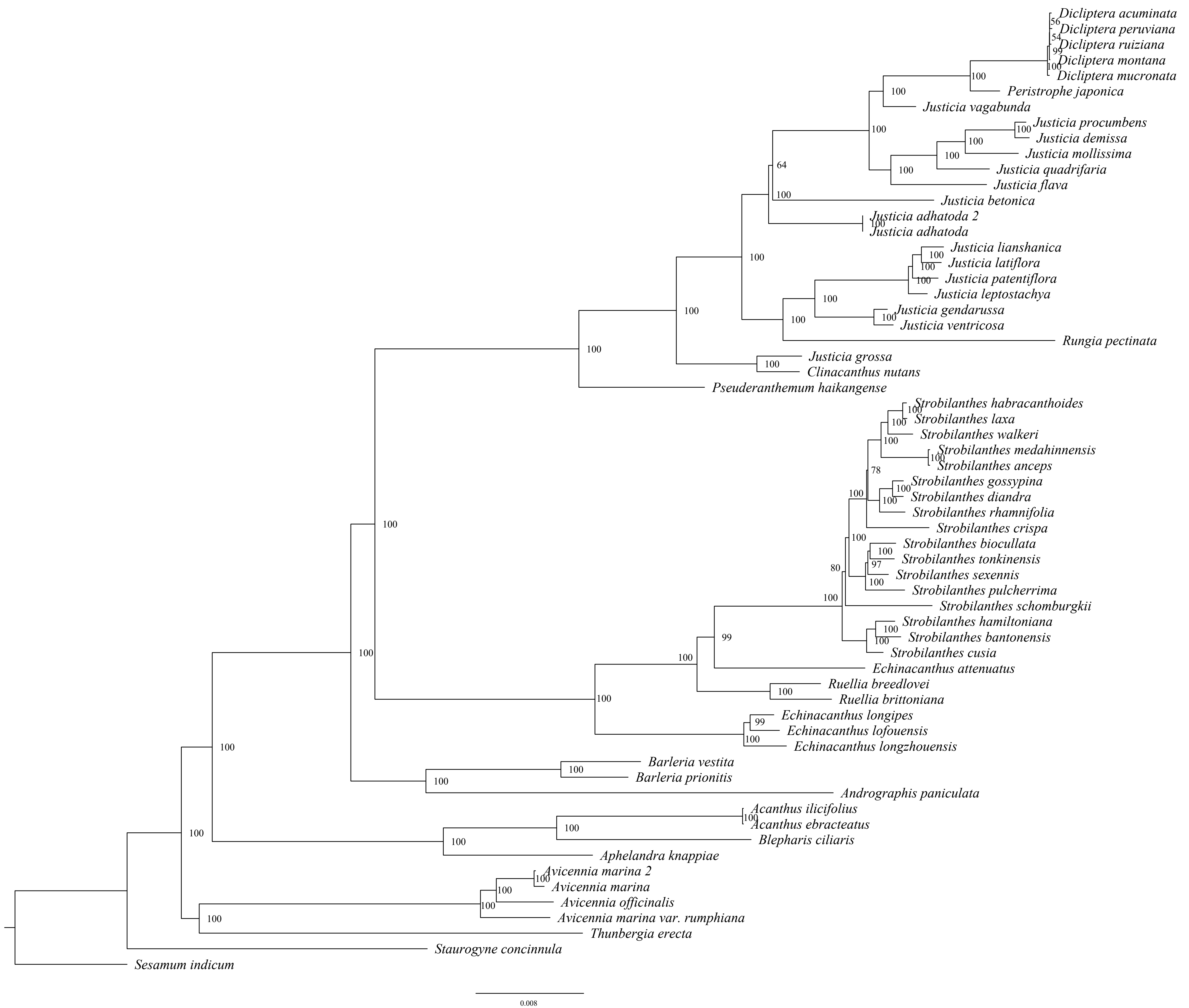
Fig. S1 ML phylogram for 62 taxa of Acanthaceae based on 77 common protein-coding genes.
