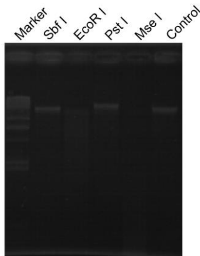
Fig. S1 Genomic DNA digested with different restriction enzyme. Marker, \lambda /Hind III DNA. Control, genomic DNA was not digested with restriction enzyme.
