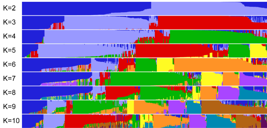
Fig. S4 Population structure analysis of 468 tea accessions with K value from 2 to 10.
