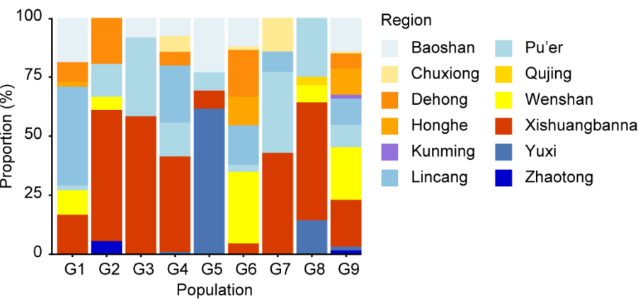
Fig. S5 The proportion of accessions from different geographic regions in each population. Different regions are represented by blocks of different colors.
