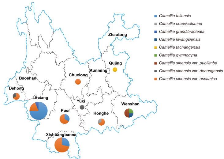
Fig. S6 Geographical distribution of the core collection in Yunnan province. The color and size of solid circle indicated the species type and number of tea accession, respectively.
