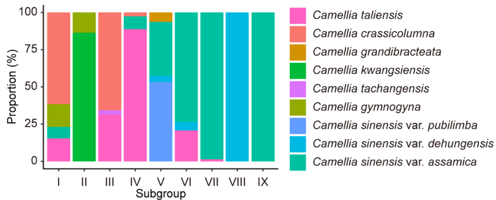
Fig. S2 The proportion of accessions in each subgroup of phylogenetic tree. Different sect. Thea species are represented by blocks of different colors.
