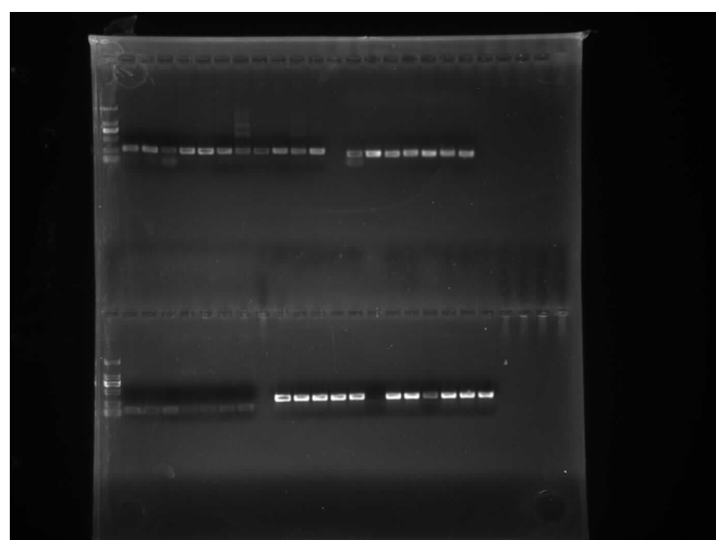
ITS
