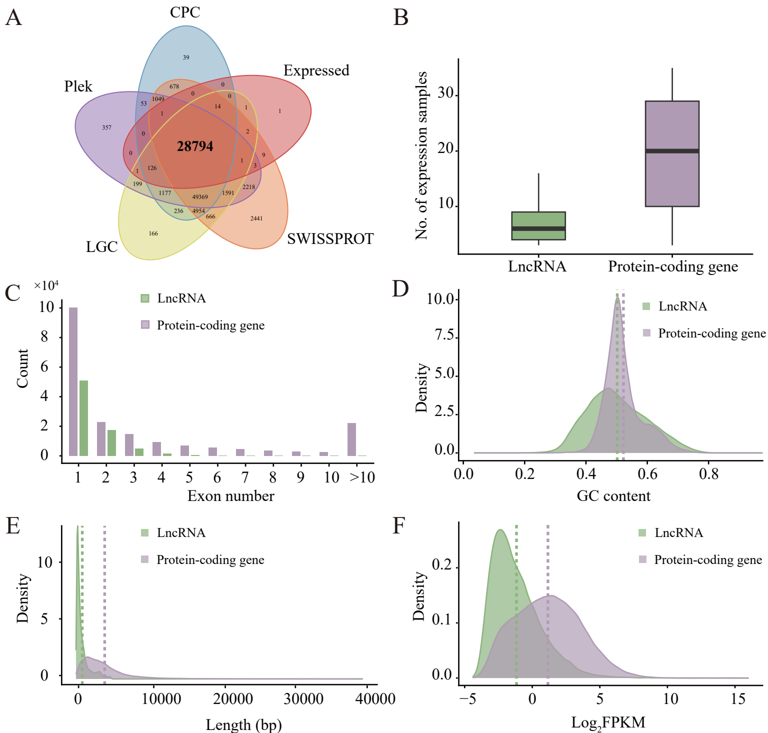
Fig. S2 Characteristics of FHB-related protein-coding genes and lncRNAs in wheat.
