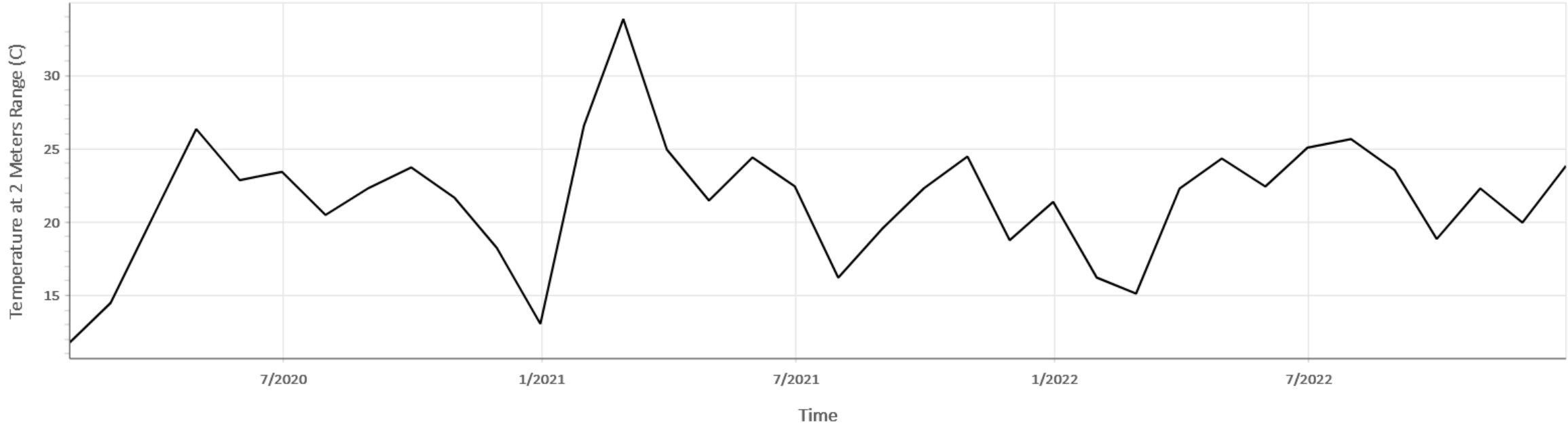
PHR Time Series of Monthly Temperature at 2 Meters Range 2020/01/01 to 2022/12/31 (Lat: 52.75, Lon: 17.14)
