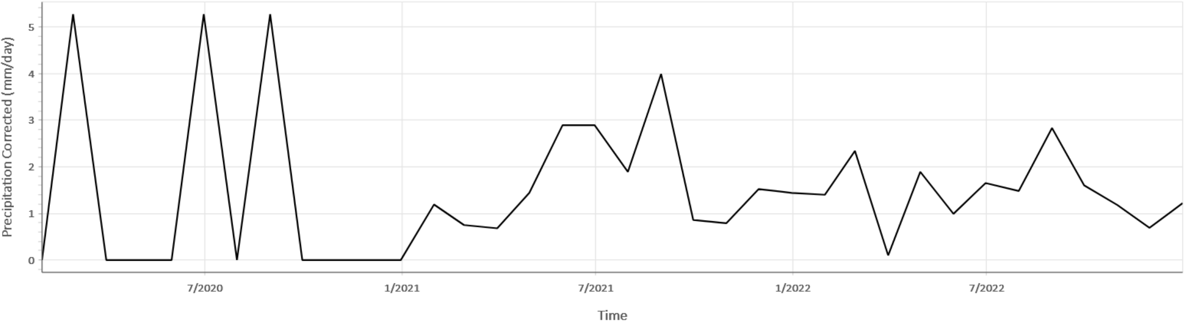
PHR Time Series of Monthly Precipitation Corrected 2020/01/01 to 2022/12/31 (Lat: 52.75, Lon: 17.14)
