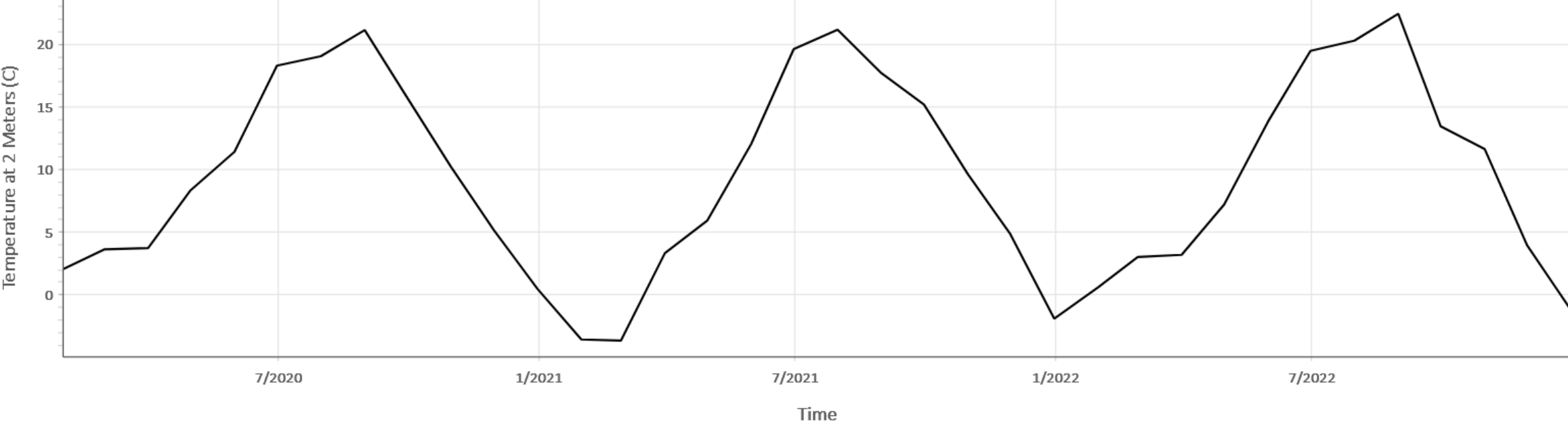
PHR Time Series of Monthly Temperature at 2 Meters 2020/01/01 to 2022/12/31 (Lat: 52.75, Lon: 17.14)
