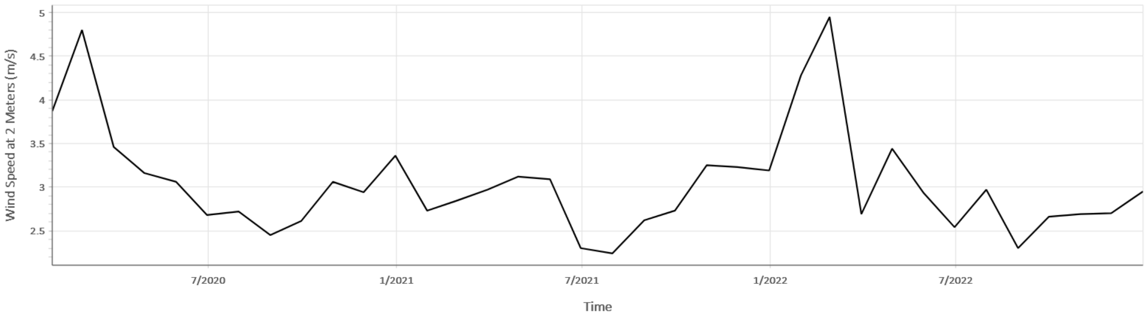
PHR Time Series of Monthly Wind Speed at 2 Meters 2020/01/01 to 2022/12/31 (Lat: 52.75, Lon: 17.14)
