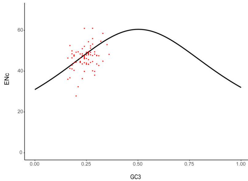
Fig S1 ENC-plot of Styrax . ENC refers to the Effective Number of Codons, which measures the degree of codon usage bias within a gene. GC3 means Guanine-Cytosine content at the third codon position, used to assess evolutionary characteristics of genes. The ENC-plot distinguishes whether the driving factor behind codon bias is natural selection or mutation-drift equilibrium.
