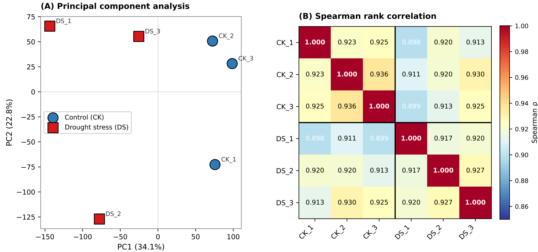
Figure S6 Principal component analysis and Spearman correlation of CK and DS RNA-seq libraries.
