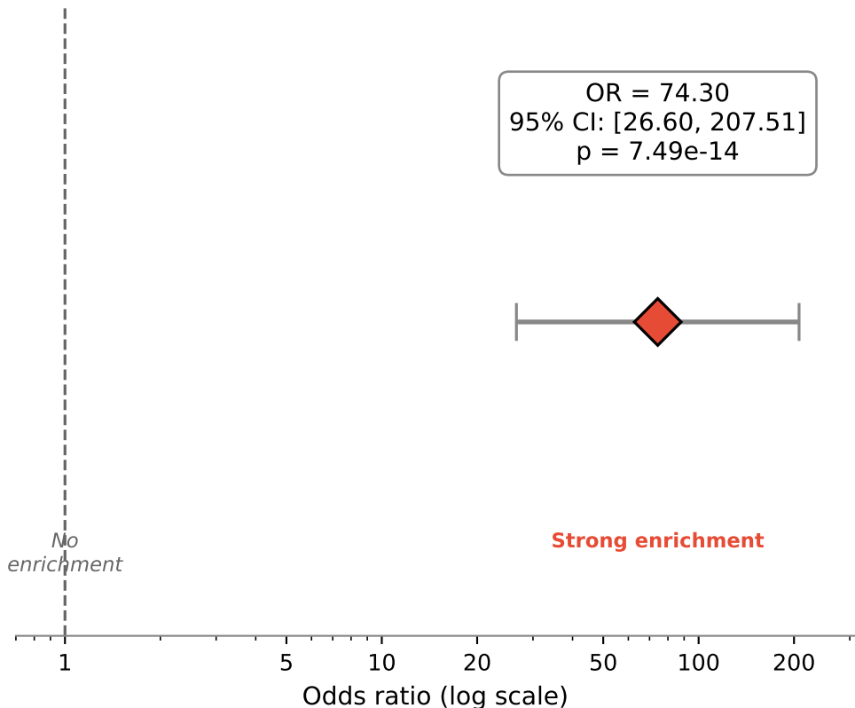
(B) FAR1/FHY3 enrichment among cis-target TFs (Fisher OR + 95% CI)
