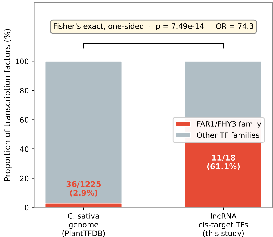
(A) FAR1/FHY3 proportion: genome vs lncRNA cis-targets
