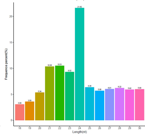
Figure S1. Proportion of miRNAde length in each sample
