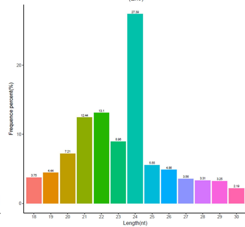
Sequence length distribution (Ca3)
