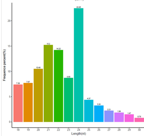
Sequence length distribution (Ca1)
