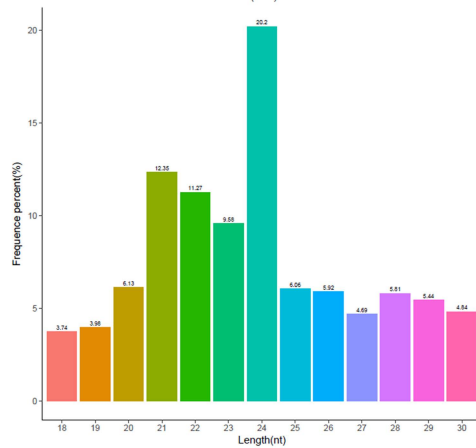
Figure S1. Proportion of miRNAde length in each sample
