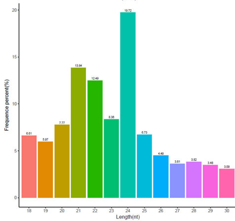
Sequence length distribution (G1)
