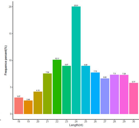
Sequence length distribution (G3)
