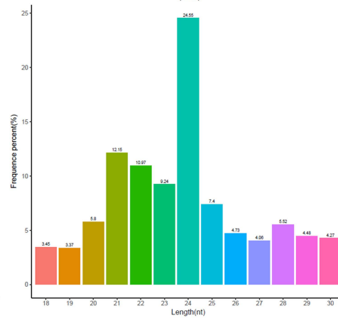
Sequence length distribution (G2)
