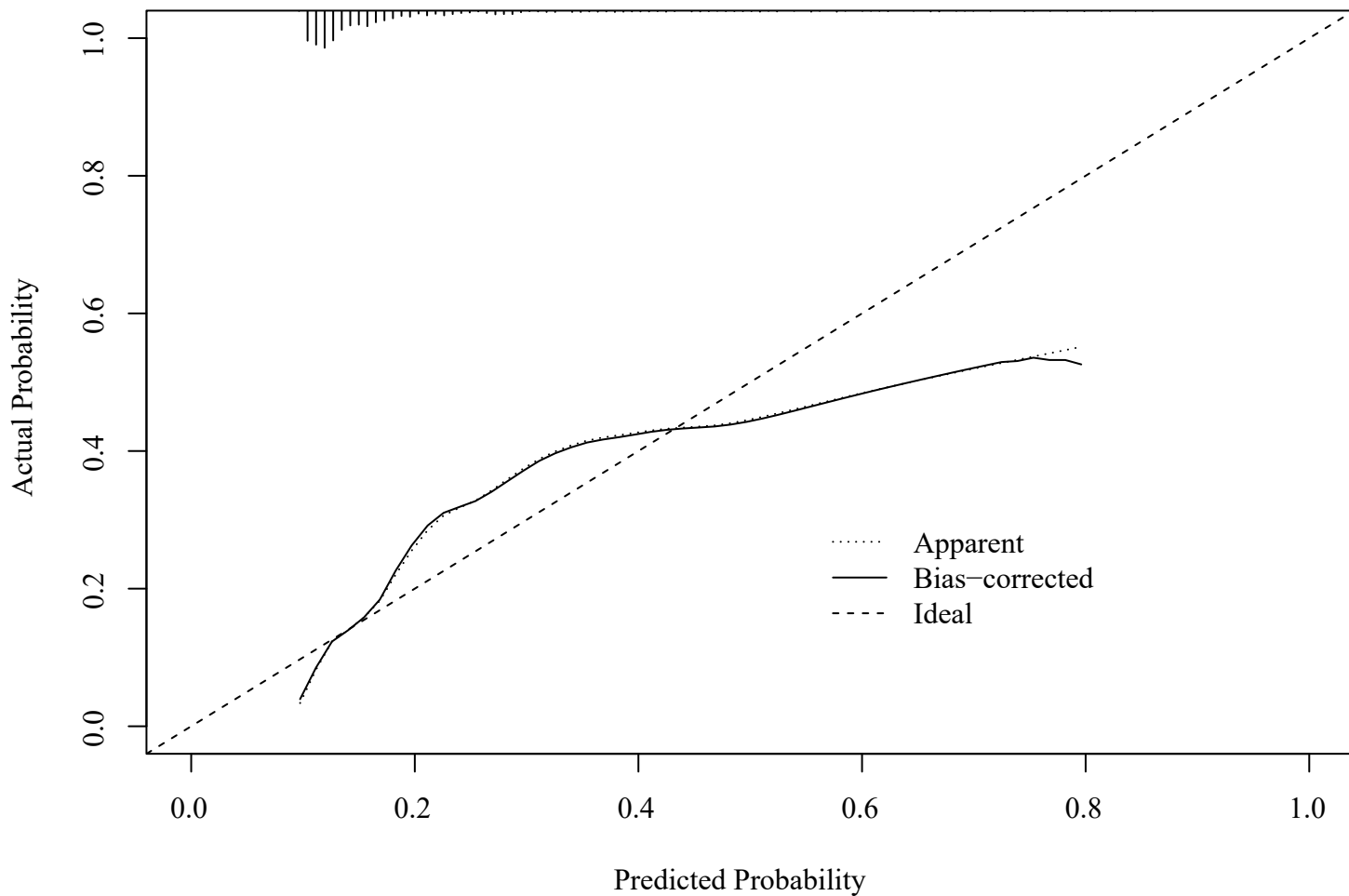
Supplementary Figure 4 The calibration curve of our prediction model in the external validation set.
