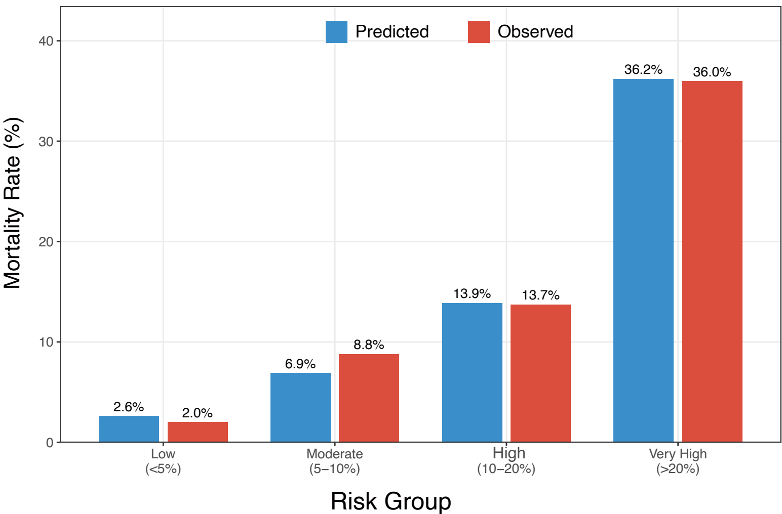
C. Predicted vs Observed Mortality by Risk Group
