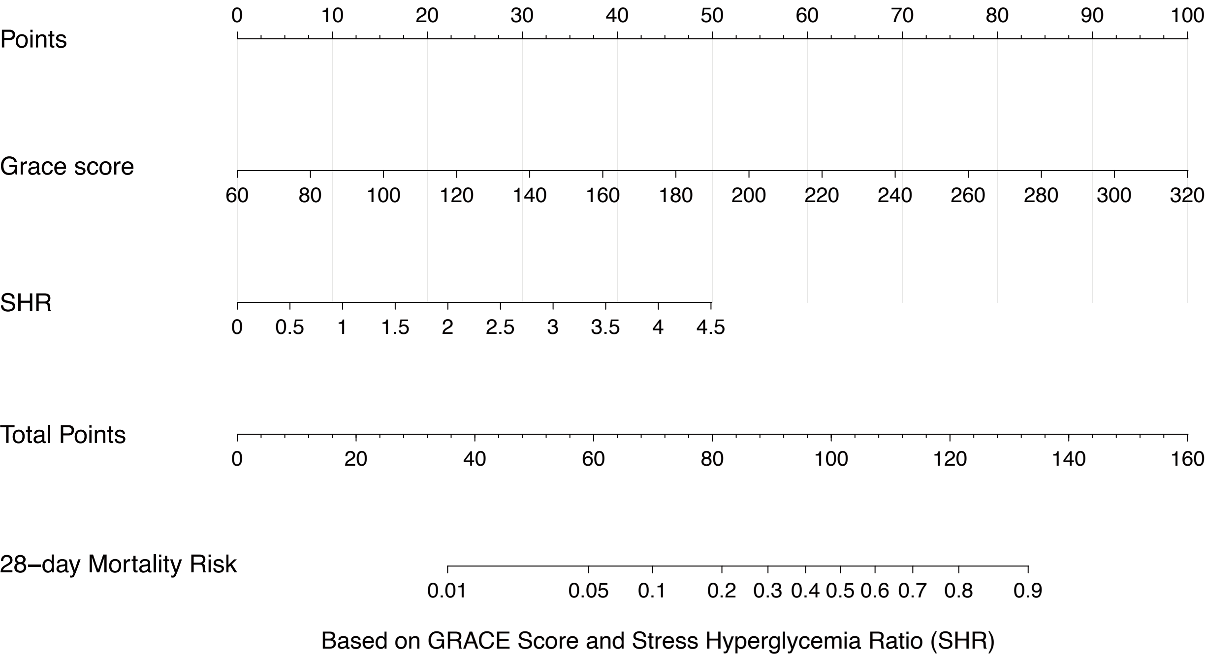
A. Nomogram for Predicting 28-day Mortality in ACS Patients
