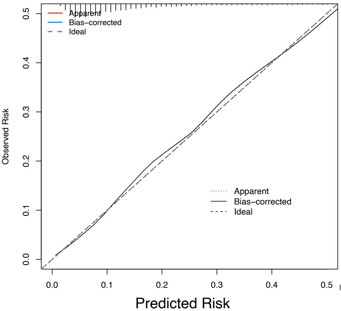
B. Calibration Plot
