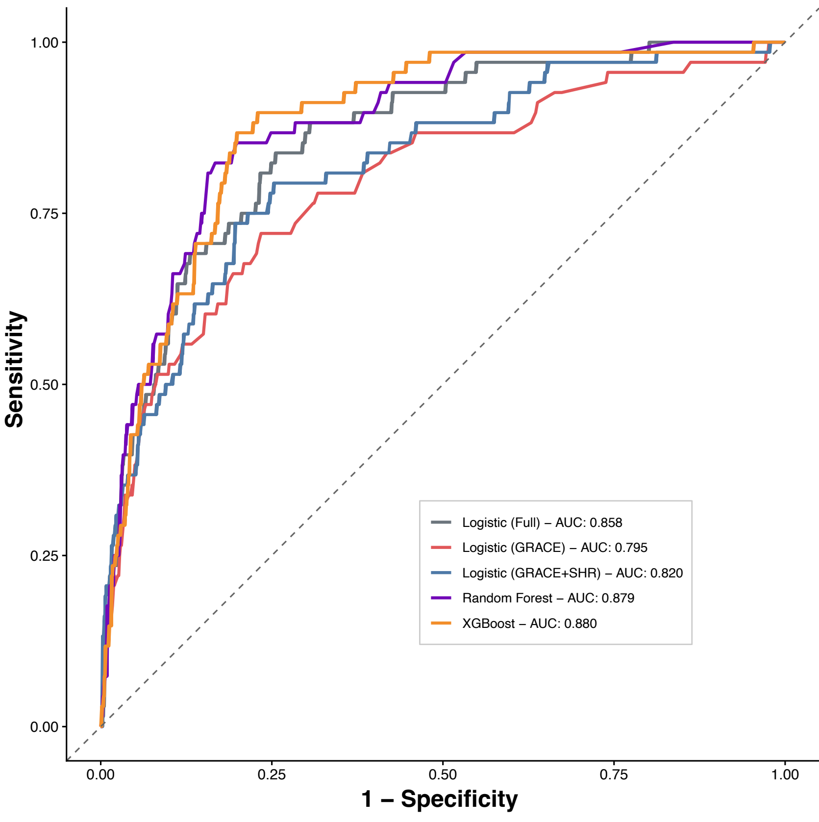
A. ROC Curves: ML Models vs Traditional Logistic Regression
