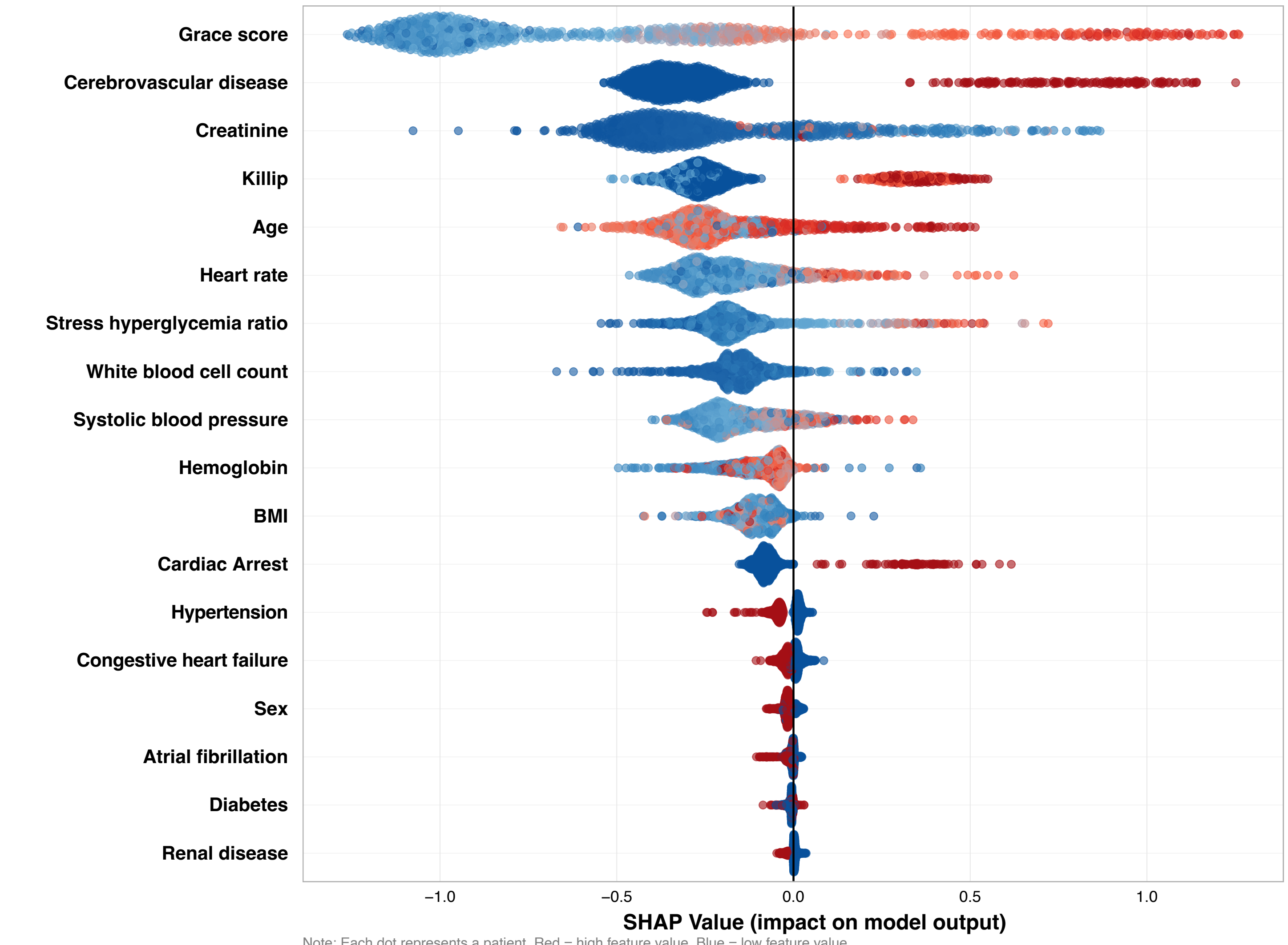
C. SHAP Feature Importance – Beeswarm Plot
