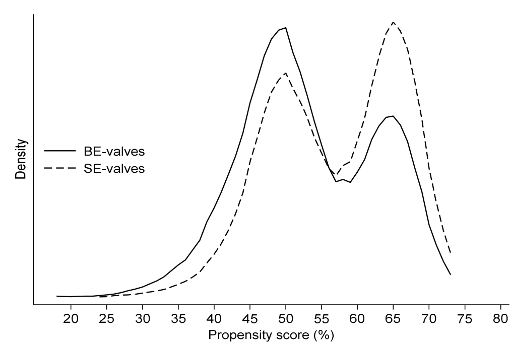
Figure S1: Overlap plot
