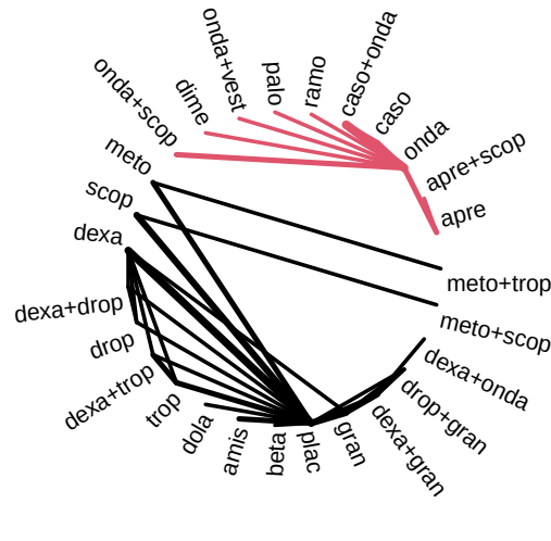
Disconnected 14 (m=56, k=38)
