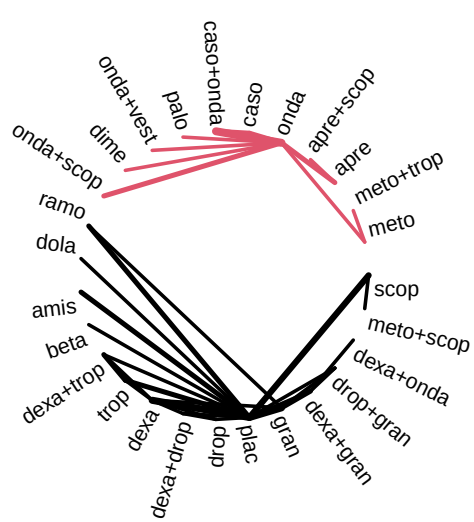
Disconnected 10 (m=58, k=38)
