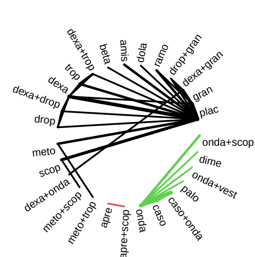
Disconnected 12 (m=57, k=37)
