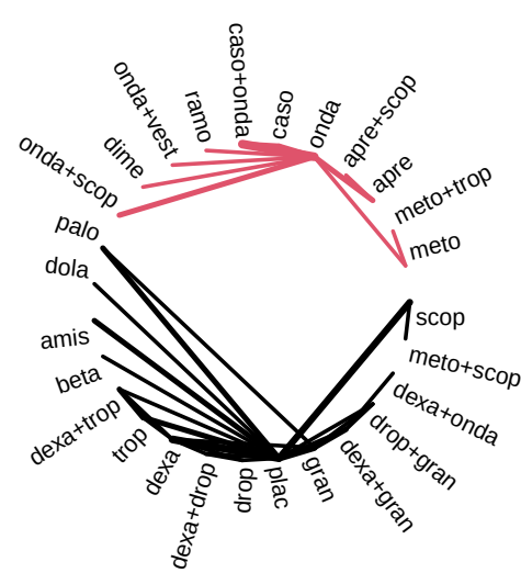
Disconnected 11 (m=57, k=39)
