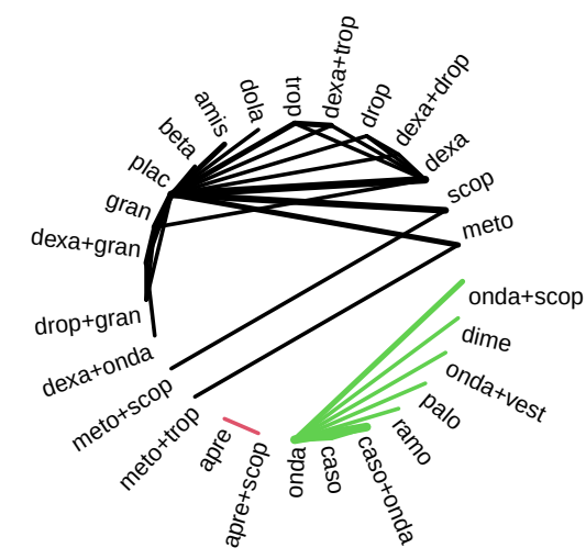
Disconnected 18 (m=54, k=36)
