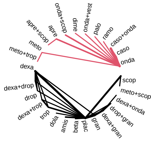
Disconnected 17 (m=55, k=37)
