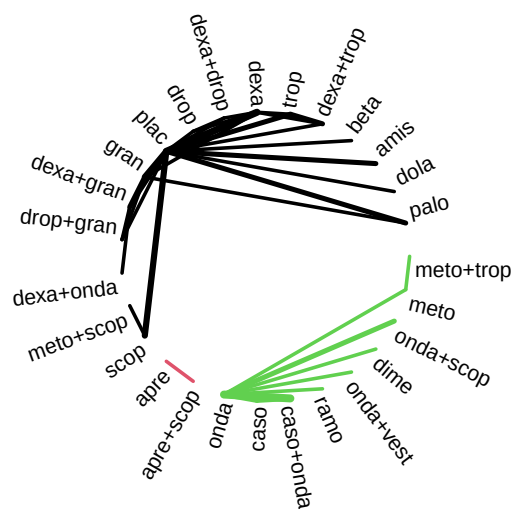
Disconnected 16 (m=55, k=37)
