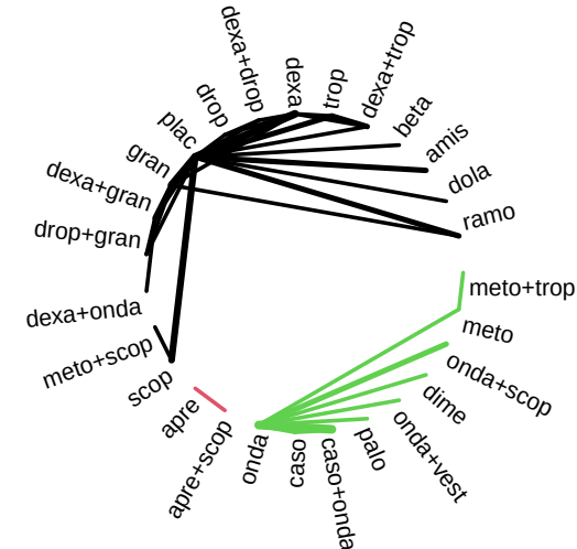
Disconnected 15 (m=56, k=36)
