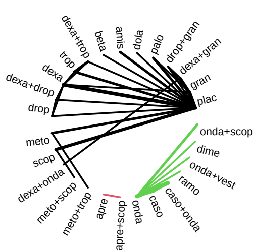
Disconnected 13 (m=56, k=38)
