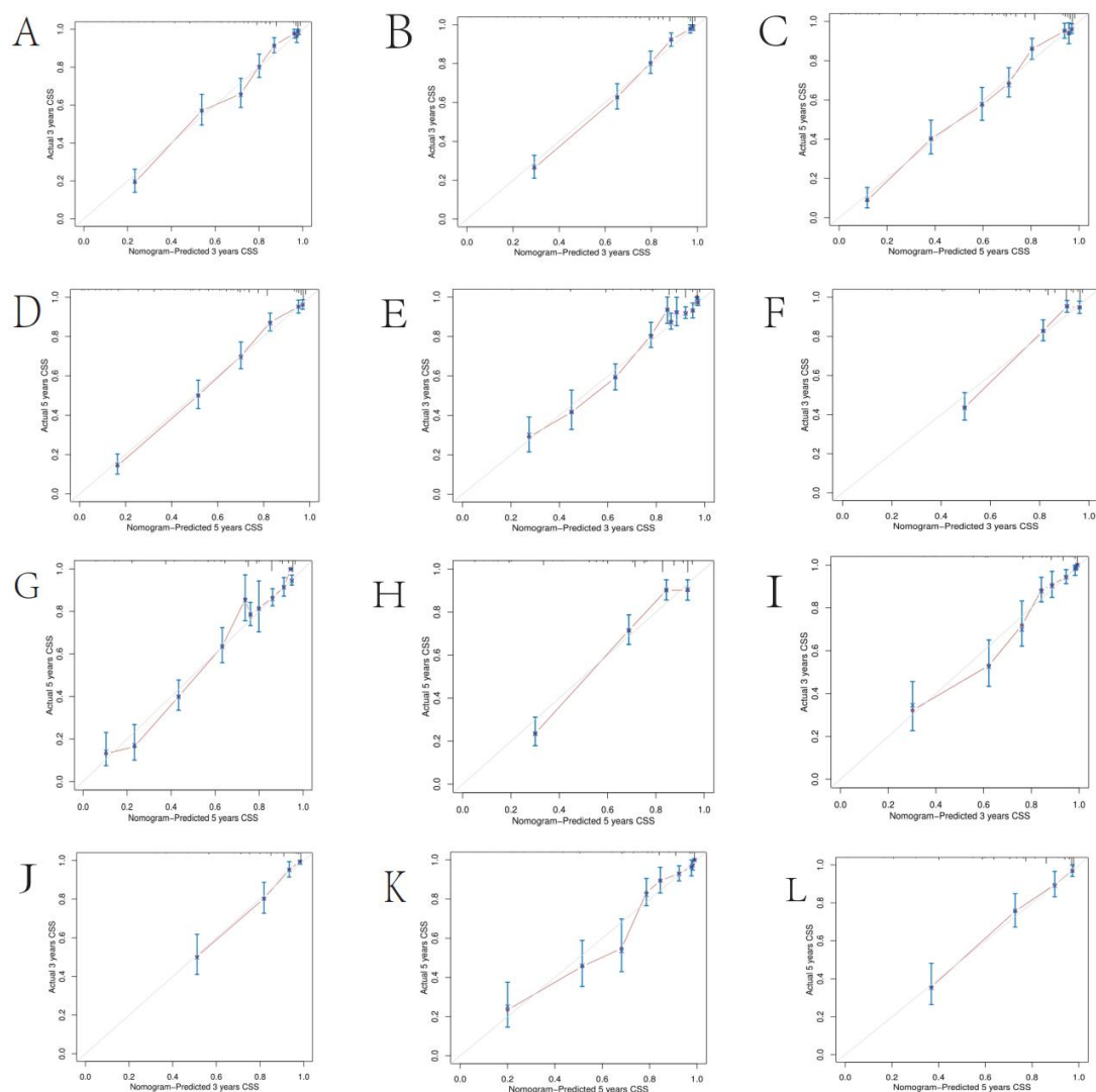
Supplementary Fig. 4 The calibration curves of the prognostic nomogram for 3-year and 5-year CSS in the training sets and validation sets in right-sided EOCC (A-D), left-sided EOCC (E-H) and transverse-sided EOCC (I-L). Abbreviations: EOCC Early-onset colon cancer, CSS Cancer-specific survival.
