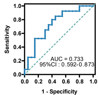
\gamma -Glutamylglutamic acid
