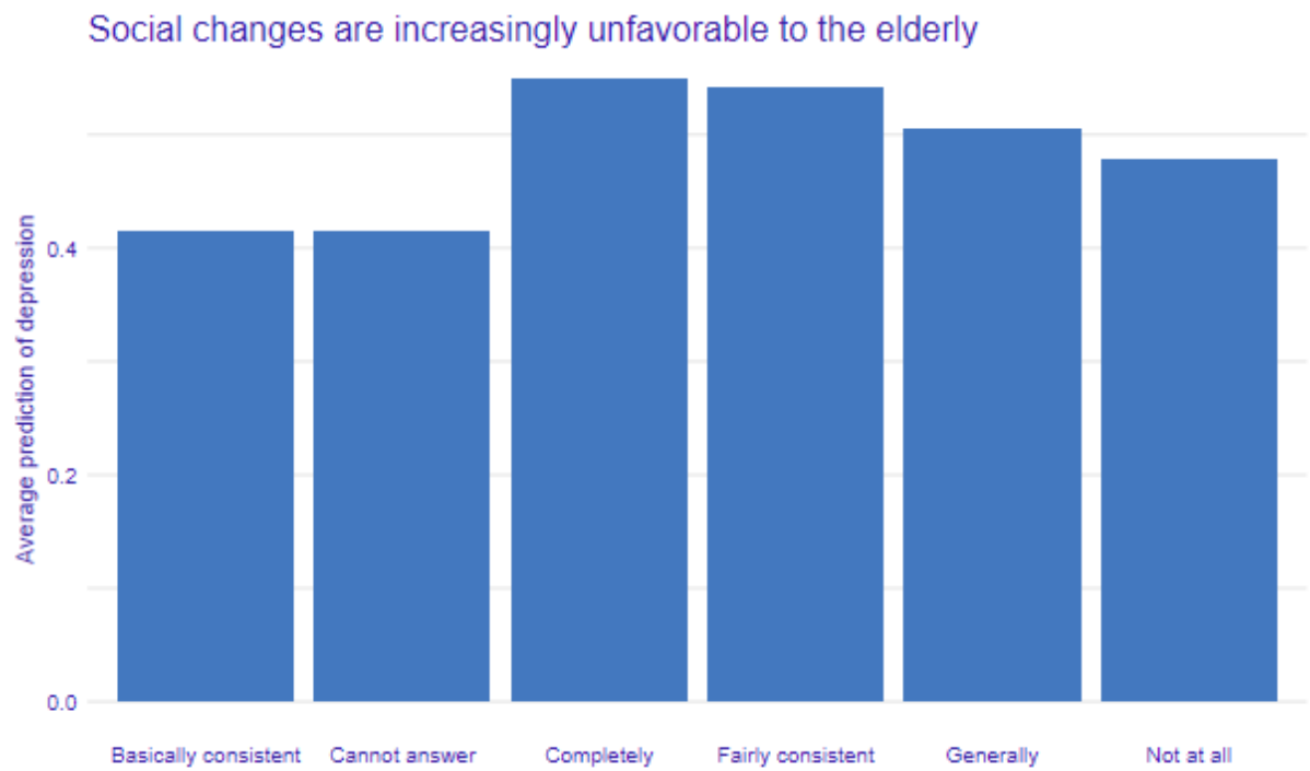
Supplementary Figure 5: Accumulated local effects plot for social change are increasingly unfavourable to the elderly
