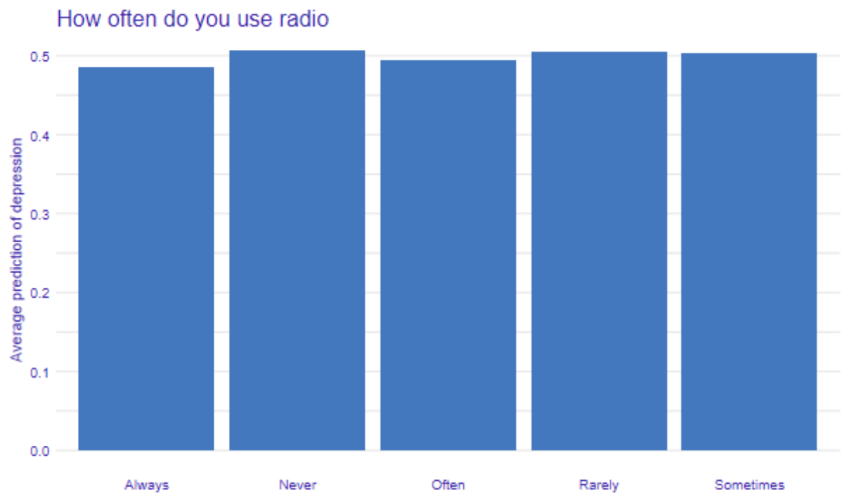
Supplementary Figure 3: Accumulated local effects plot for how often do you use radio
