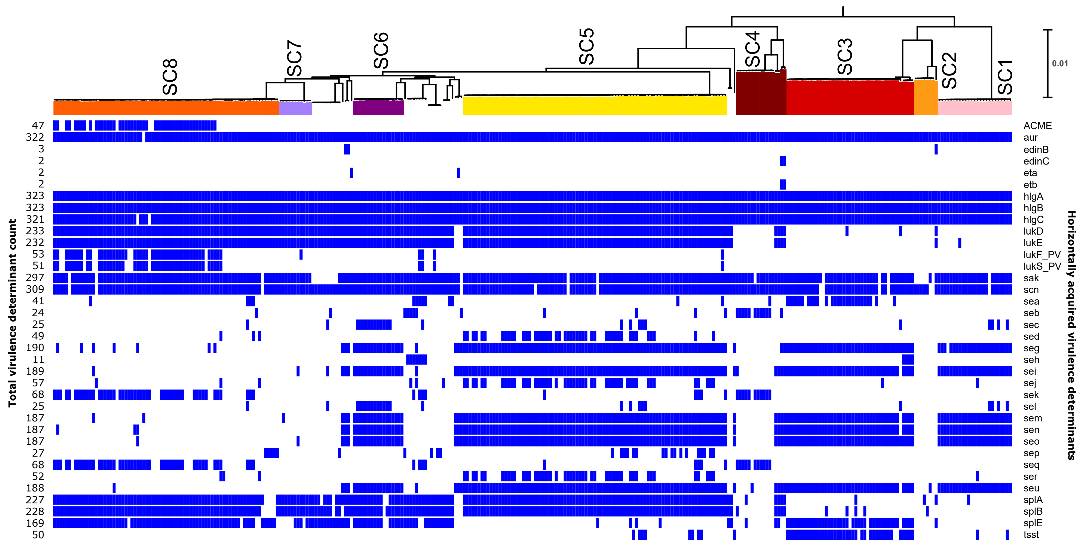
Figure S3: Distribution of virulence genes using VirulenceFinder and the Virulence Factor Database (VFDB). Details are shown in Supplementary Table S4.
