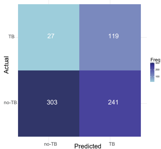
E RF Model Confusion Matrix
