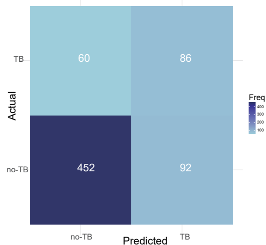
D NB Model Confusion Matrix
