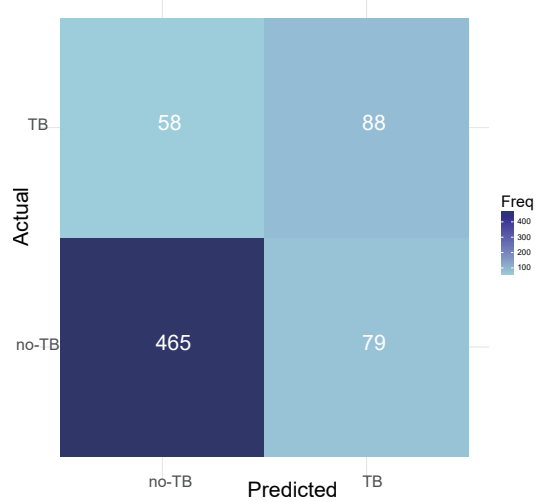
G Xgboost Model Confusion Matrix
