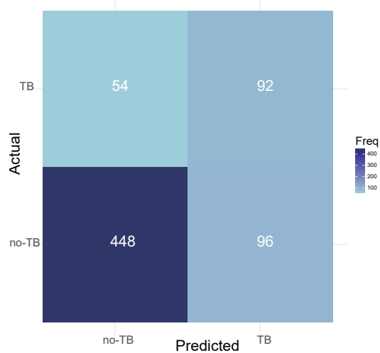
F SVM Model Confusion Matrix
