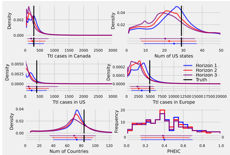
Figure S2: Human judgment ensemble predictive densities one (blue), two (red), and three (purple) weeks ahead of the date of the true value (black vertical line). Below each plot is presented a 25th quantile (leftmost point of the line), 50th quantile (dot), and 75th quantile (rightmost point of the line).
