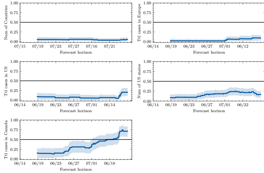
Figure S3: The proportion plus 95% confidence intervals of individual median predictions that were greater than the ground truth for five continuous targets from three weeks before the ground truth to one week before the ground truth in intervals of one hour. The majority of human judgment forecasters submitted densities with a median below the ground truth. Only when asked to predict the total number of cases in Canada did human forecasters over estimate the severity of the mpox outbreak.
