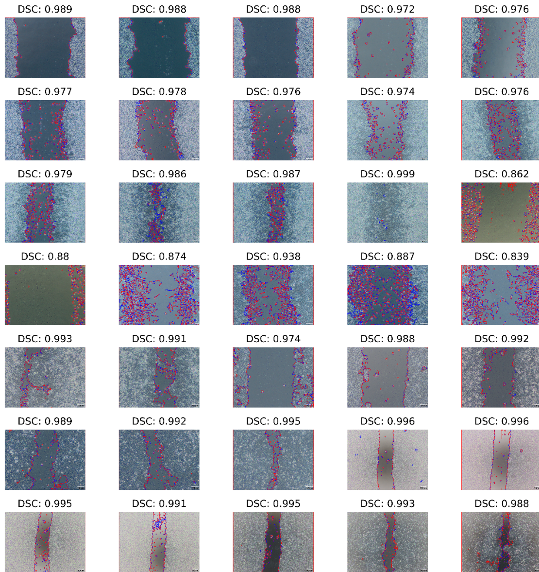
Additional File 3. – Figure A3: Validation phase results for Attention U-net model. Each validated image sample showed as in its original form, and the predicted and ground truth labels contours were drawn on the image to observe the edge prediction discrimination. Contour lines were denoted as Red (-) for Predicted and Blue (-) for Ground-Truth (DSC: Dice Similarity Coefficient).
