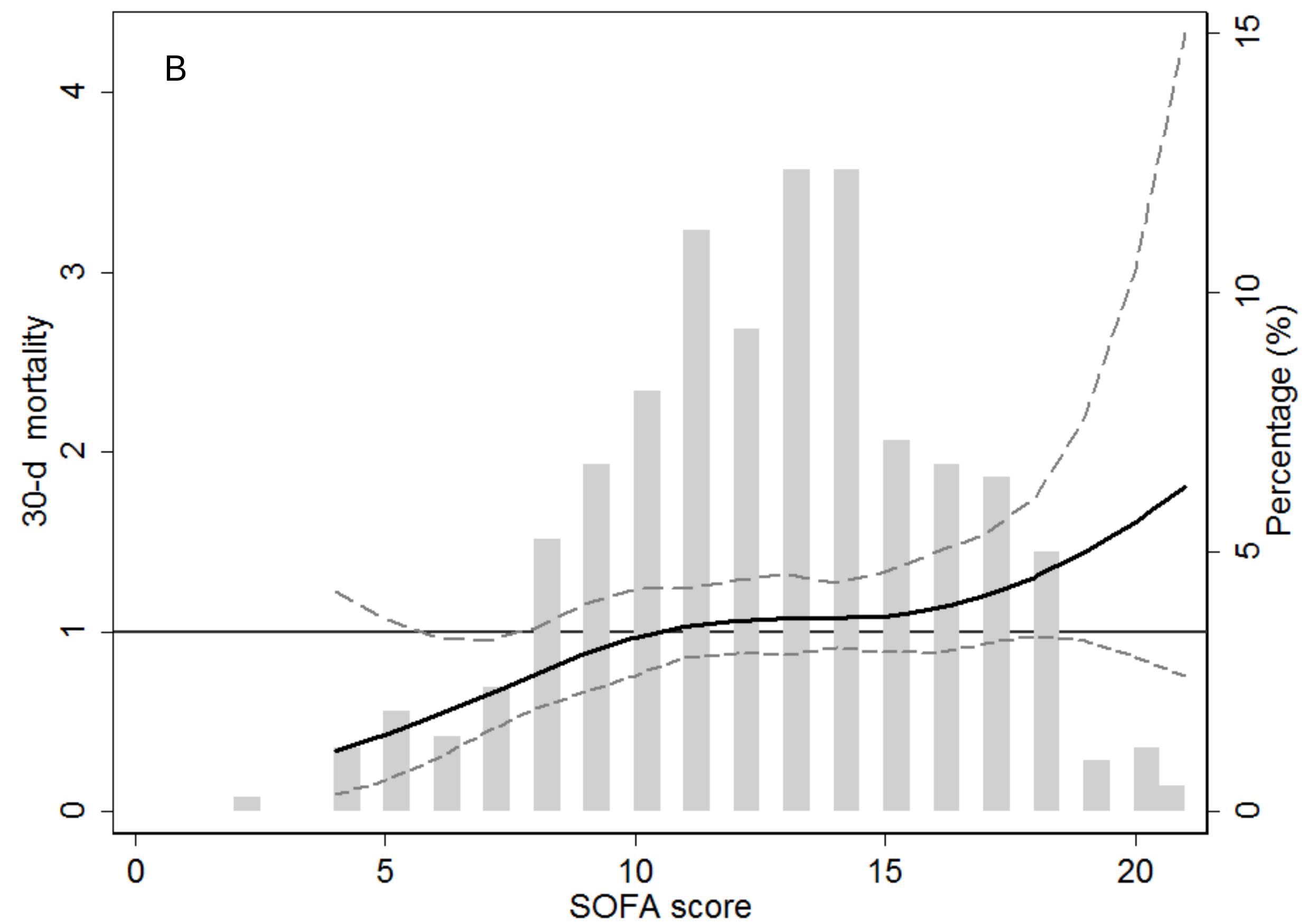
Figure S1. The cubic spline curves for 30-day mortality according to SOFA score. (a) non-obese group, (b) obese group, Abbreviations: SOFA, sepsis-related organ failure assessment
