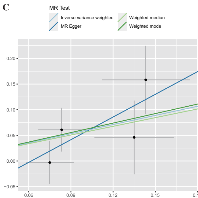
Supplementary Figure 2. Forest plot (A), sensitivity analysis (B), scatter plot (C), and funnel plot (D) of the causal effect of Adlercreutzia on UIA risk.
